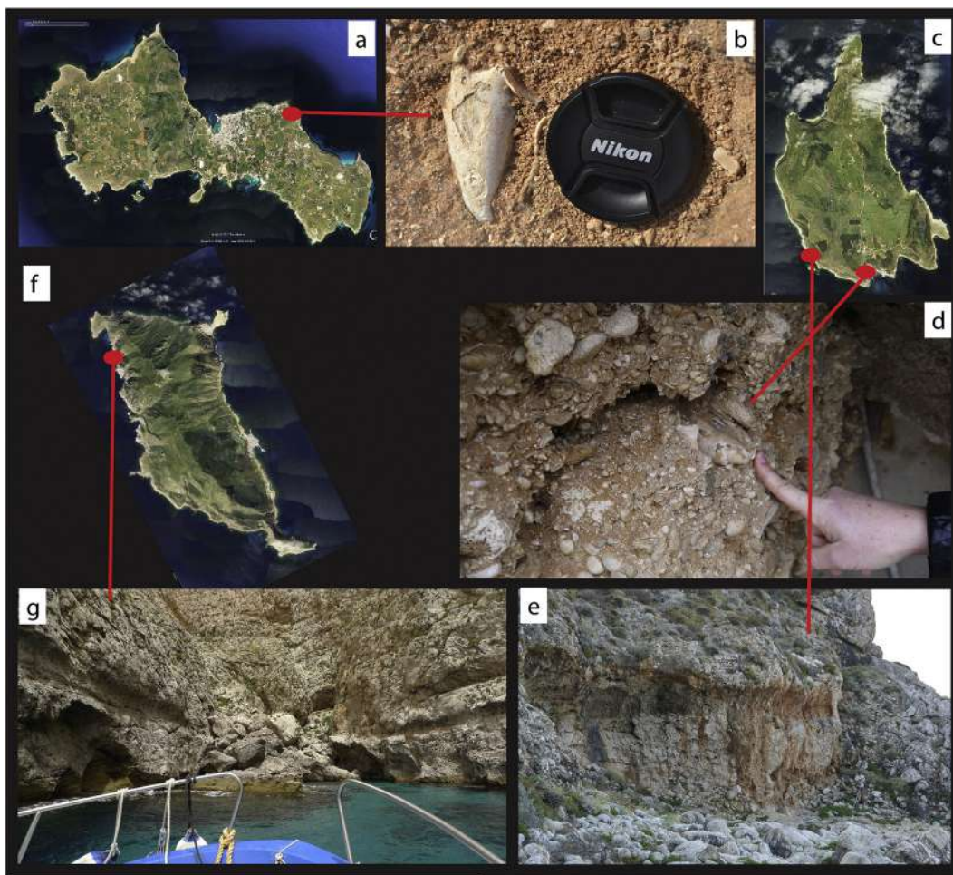
Fig. 3. MIS 5.5 highstand evidence on the Egadi archipelago: (a) Favignana, (b) MIS 5.5 deposit with Persistrombus latus , (c) Levanzo, (d) MIS 5.5 deposit with Persistrombus latus , (e) MIS 5.5 tidal notch, (f) Marettimo and (g) MIS 5.5 tidal notch.
