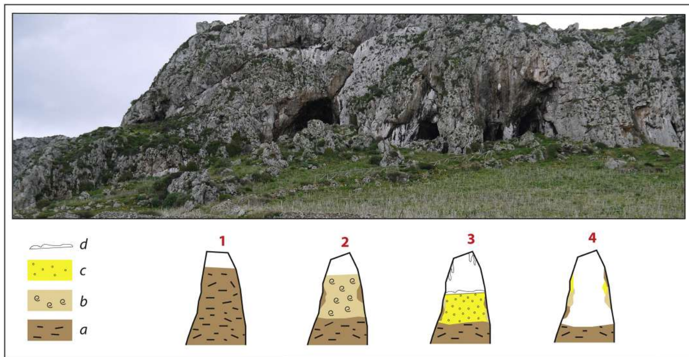
Fig. 5. Summary sketch of the filled fossil sediments and geomorphological evolution of the caves of Ucceria (Punta Faraglione). (a) Aeolin sands sealing Lithophaga of Middle Pleistocene, (b) silty sands containing Pulmonata shells, (c) coarse sands and well-cemented breccias containing copious fossil meal remains ( P. ferruginea , Monodonta , but also bones and teeth of large mammals) and (d) flowstone that seals the previous deposit.
