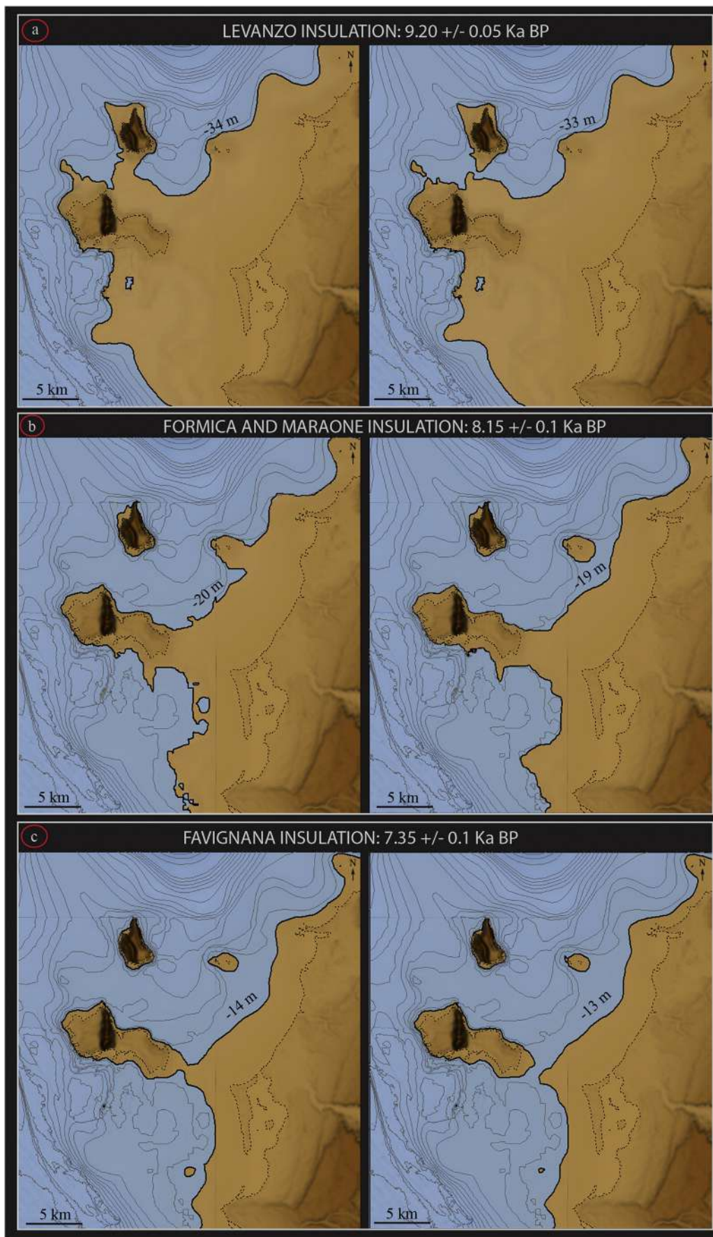
Fig. 12. Levanzo, Formica, Maraone and Favignana insulations.
