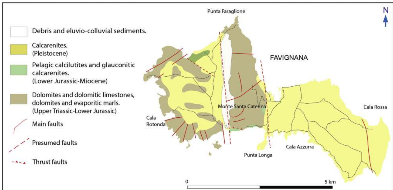
Fig. 2. Geological sketch of the Egadi archipelago simplified from Abate et al. (1997).
