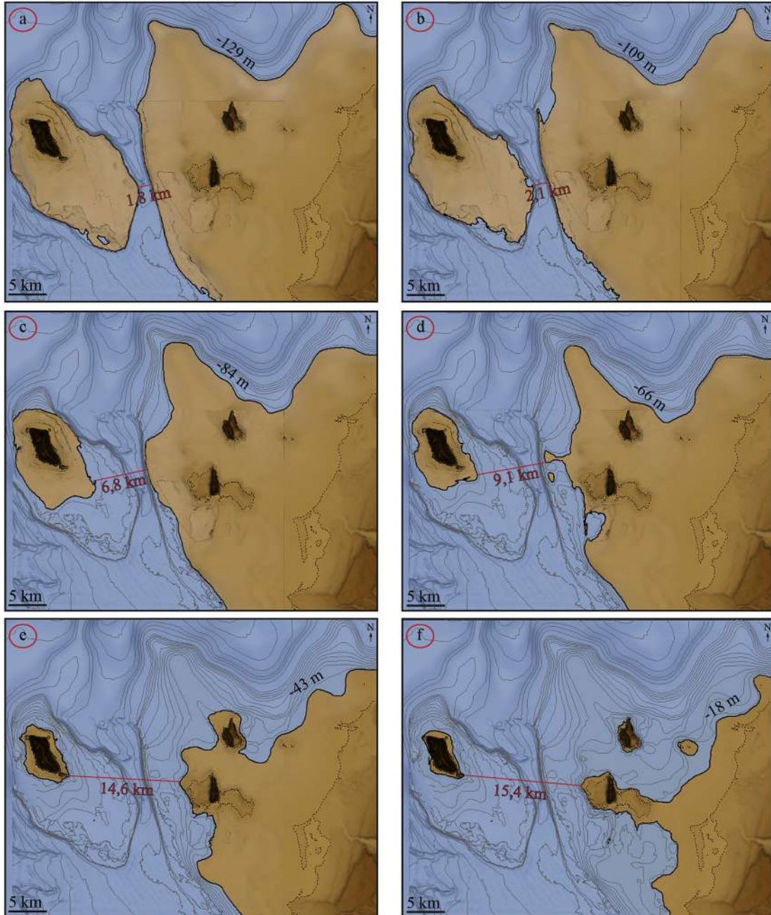
Fig. 11. Palaeoshoreline reconstruction of the Egadi and Sicily Islands from the LGM to the present day.
