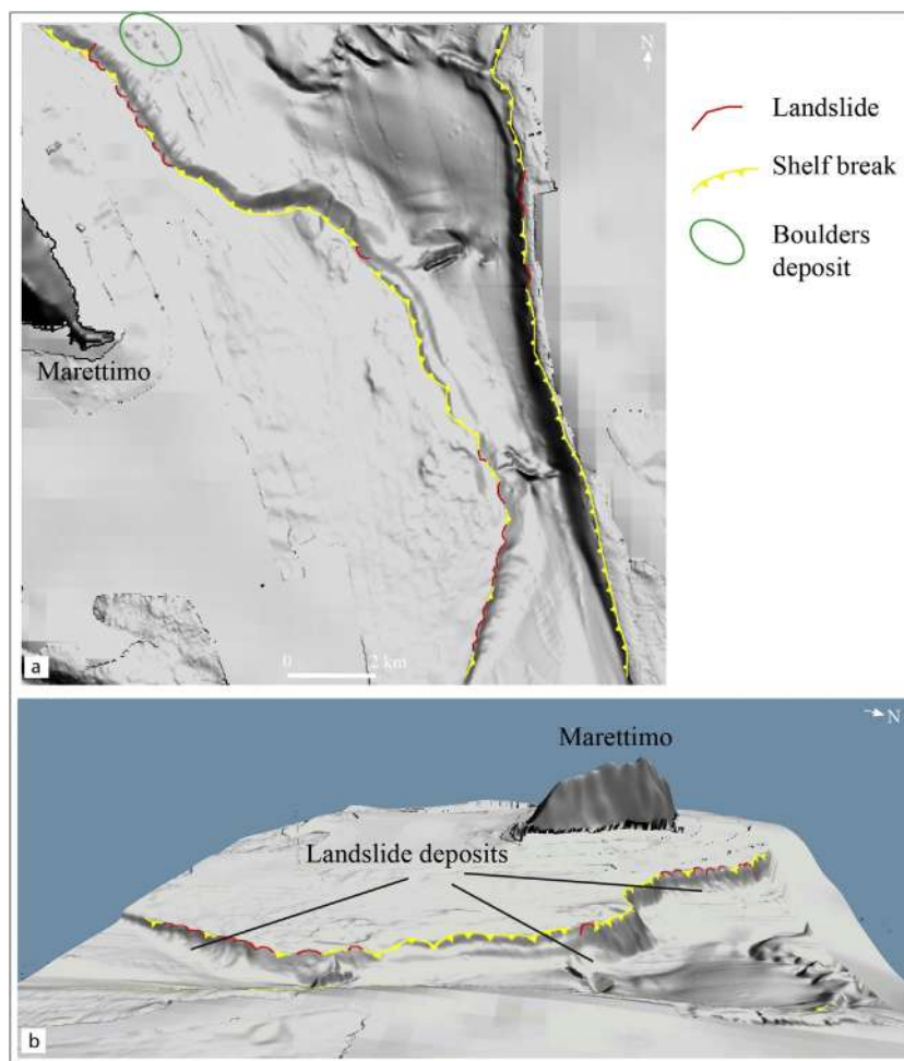
Fig. 9. Morphobathymetric data: Marettimo canyon, canyon shelf break, submerged landslide, landslide deposits and boulders deposits.
