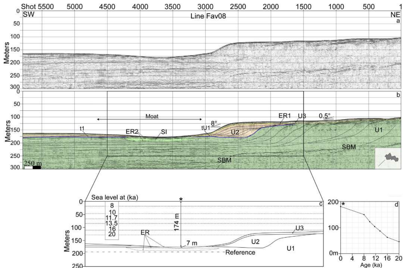
Fig. 10. Southwest-northeast high-resolution seismic reflection profile (a) across the Marettimo canyon. The geoseismic interpretation (b) shows the Lower-Middle Pleistocene progradational to aggradational sequence (U1), covered by the LIPW (U2) and the transgressive-highstand system tracts (U3) pertaining to the Upper Pleistocene depositional sequence. In the geological sketch (c), the present-day position of the canyon thalweg (*) points out. At this point, we reconstructed the progressive increase in water depth (d) until 20 ka cal BP, taking into account sea-level rise, sedimentation rate and erosional processes.
