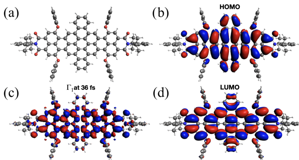
Figure 8. Induced density of DNQDI (a). The calculated time-resolved induced density (c) is shown, compared with HOMO (b) and LUMO (d). Snapshot at 36 fs.
