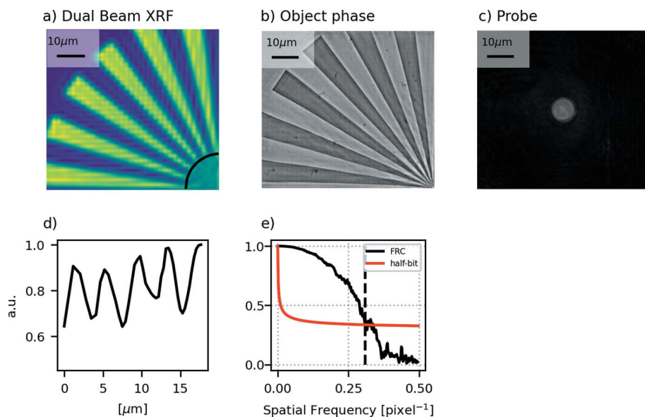
Figure 4 Ptycho-fluorescence results: (a) Fluorescence image of the Siemens star obtained with dual beam setups. (b–c) Ptychographic reconstruction of the phase image of the Siemens star and probe modulus obtained with the energy filtered data. Reconstructed pixel size: 77 nm. (d) Line profile for the fluorescence image showing the resolution of 4 μm limited by the smallest beam size D_2 = 2 \mu\text{m} . (e) Fourier ring correlation analysis for the ptychography reconstruction showing a resolution of 0.31 \text{ pixel}^{-1} , corresponding to 248 nm.
