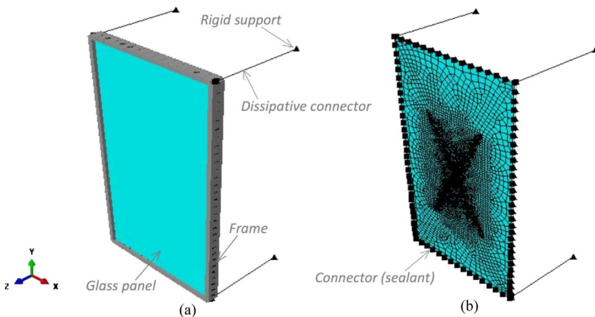
Fig. 8. FE model assembly and features. (a) Extruded view and (b) overview of mesh patterns and mechanical connectors (ABAQUS [73]).
