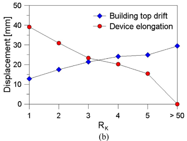
Fig. 10. Seismic dynamic analyses on the 3D steel building with UGCWs. (a) Set of natural seismic spectra, as derived from the REXEL software [77]; (b) effect of vibration control devices on the examined building, with evidence of top drift and relative device sliding, as a function of R_K (ABAQUS [73]).
