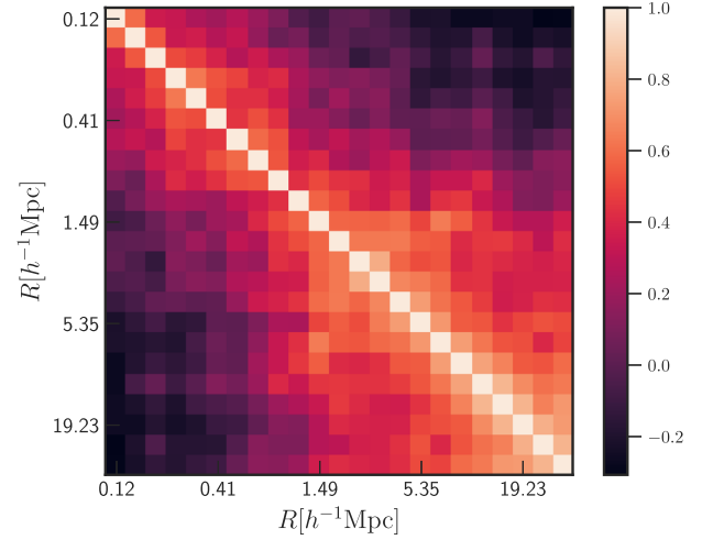
Figure D1. The normalized covariance matrices for \Delta\Sigma(R) (top, see Section 3.2) and \Sigma_g(R) (bottom, see Section 3.4). Note that the covariance matrix for \Delta\Sigma(R) includes the boost factor correction (see Section 3.3).
