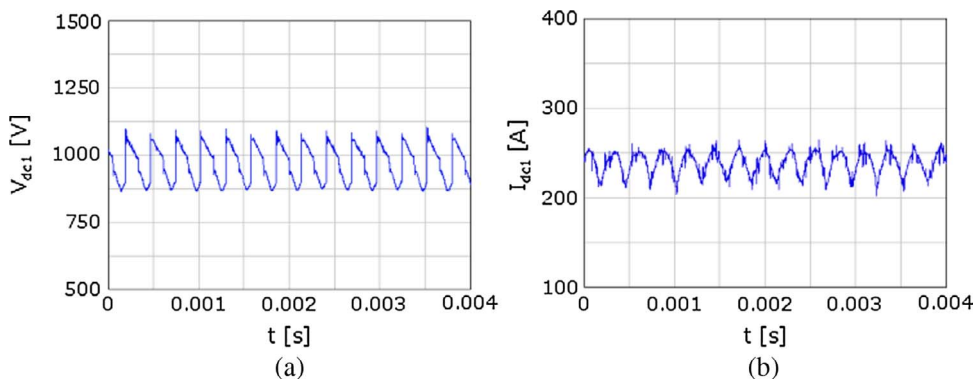
Fig. 7. Measured output quantities of the diode rectifier: (a) voltage ( V_{dc1} ), (b) current ( I_{dc1} ).
