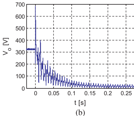
Fig. 3. Effects of an experimental short circuit test at the output terminals of one diode bridge of a DC power generator composed of two series-connected diode bridges fed by a double three-phase synchronous machine: (a) recorded current, (b) recorded voltage.
