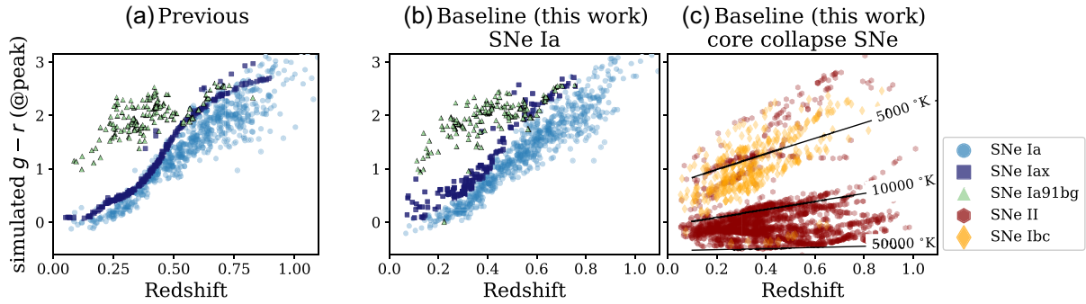
Figure 4. Simulated g - r colours at peak brightness for various types of SNe as a function of redshift. In panel (a), SNe Ia are generated using the SALT2 SED model from Betoule et al. (2014), and SNe 91bg and SNe Iax using the original PLAsTiCC templates. In panel (b), SNe Ia are generated from the SALT2 SED model, and SNe 91bg and SNe Iax are simulated using the PLAsTiCC templates with the addition of dust extinction for SNe Iax and stretch diversity for SNe 91bg (see Section 4.3). In panel (c), core-collapse SNe are simulated using the V19 templates that include dust extinction as measured in the original events. This is the baseline simulation implemented in this analysis. For comparison with the g - r colour evolution of core-collapse SNe, we also show the g - r colour measured from blackbody SEDs at temperatures of 5000, 10 000, and 50 000 K.
