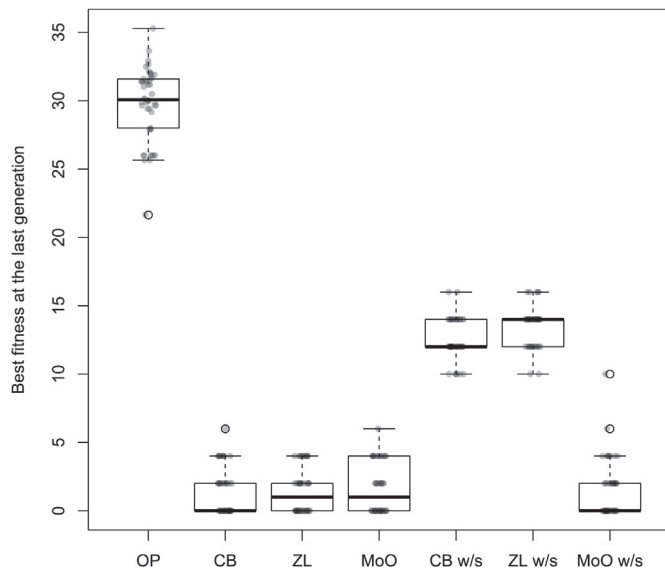
Fig. 7. Results of the OA problem, (16, 8, 2, 4) instance.
