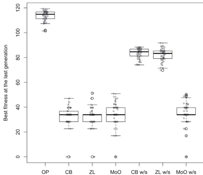
Fig. 8. Results of the OA problem, (16, 8, 3, 2) instance.
