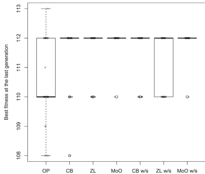
Fig. 3. Results of the Balanced Boolean functions problem, n = 8 instance.
