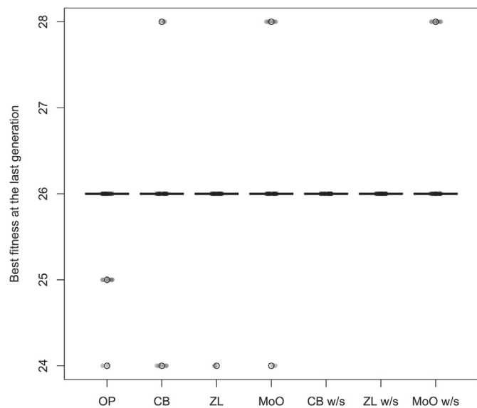
Fig. 4. Results of the bent functions problem, n = 6 instance.
