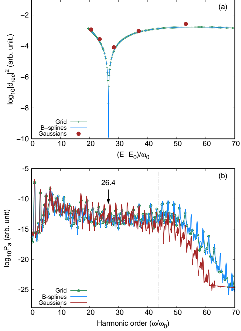
FIG. S27: Two-center interferences at R = 2.0 au: (a) recombination acceleration and (b) HHG spectrum acceleration at I = 2 \times 10^{14} W/cm ^2 . The arrow points to the expected position of the two-center interference minimum extracted from the recombination acceleration. The dot dashed line is the cutoff energy E_{\text{cutoff}} = 43.8\omega_0 .
