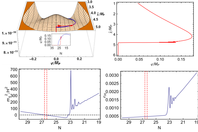
FIG. 4. Top left: the two-field potential (21) in the vicinity of the critical point (55) superimposed by the background trajectory (red) and the \varphi^+ solution (blue). Top right: the parametric plot showing \varphi(\hat{\chi}) . Bottom left: the effective isocurvature mass as a function of N . Bottom right: the slow roll parameter \varepsilon_H as a function of N . The vertical red dashed lines in the bottom row mark the beginning and end of stage 2 which lasts for less than 1e -fold. The actual fall into the valley leading to the spike in the slow-roll parameter and the isocurvature mass occurs well inside stage 3.
