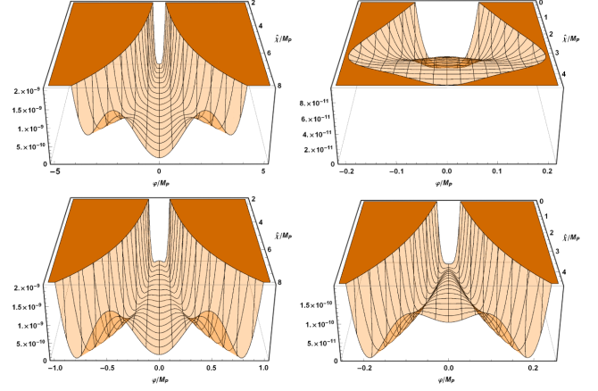
FIG. 1. The landscape of the two-field potential (21) (left column) and the vicinity of \hat{\chi}_c (right column) in scenario I (top row) and scenario II (bottom row), respectively.
