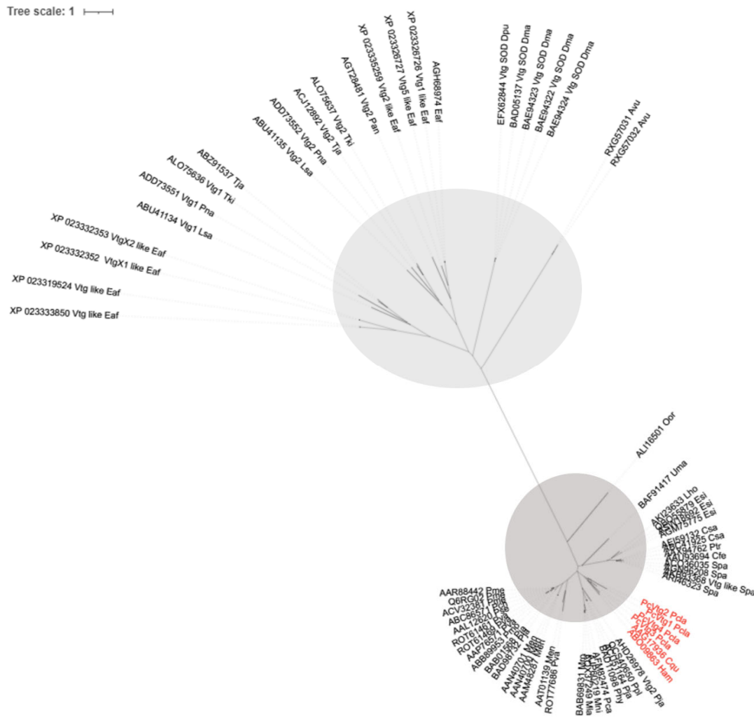
Figure 2. PhyML tree of complete VTGs stored in GenBank (until July 4, 2021). Each sequence is labelled with the corresponding GenBank ID followed by a three-character code: the first letter represents the genus name and the other two the species. P. clarkii VTGs characterized in the present study are indicated in red. In light grey is selected the cluster of Cladocera, Isopoda and Copepoda, while in dark grey the cluster of Decapoda.
