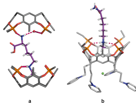
Figure 7. Side view of the molecular structures of 2H1- N ε -Me-Lys·HCl (a) and H3- N ε -Me-Lys·HCl (b) complexes. Dashed lines depicted in magenta indicate hydrogen bonding interactions.
