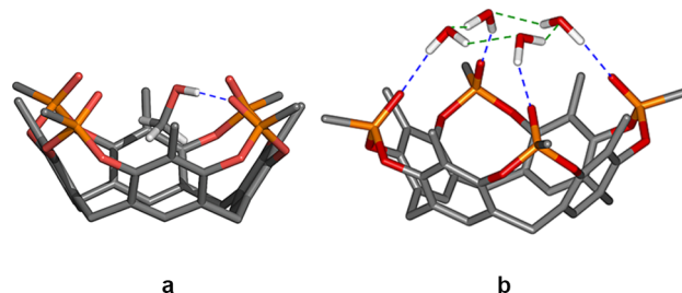
Figure 6. (a) Side view of the crystal structure of H1·MeOH. 24 The dashed blue lines indicate hydrogen bonding between the cavitaands and methanol. (b) Side view of the crystal structure of H1·4H 2 O. 22 The dashed lines depicted in blue indicate hydrogen bonding between the cavitaand and water, while water–water interactions are depicted in green.
