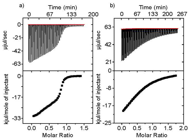
Figure 8. ITC experiments: (a) methanol, H2 = 1.04 mM, N_\epsilon -Me-Lys-HCl = 6.74 mM; (b) water, H3 = 1.69 mM, N_\epsilon -Me-Lys-HCl = 13.78 mM. The host was placed in the cell and the guest in the syringe. Top trace: raw data for the ITC titration. Bottom trace: binding isotherm of the integrated calorimetric titration data.
