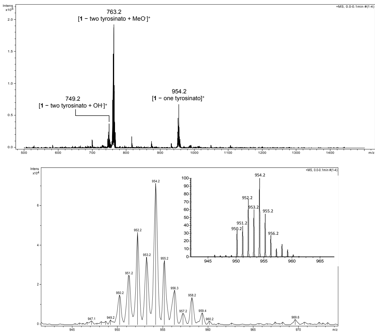
Figure S4. Top: ESI-MS ( m/z ) (positive mode) of 1 . Bottom: experimental and calculated (program IsoPro3, inset) isotopic distributions of the [1 - one tyrosinato] + peak centered at m/z 954.2.
