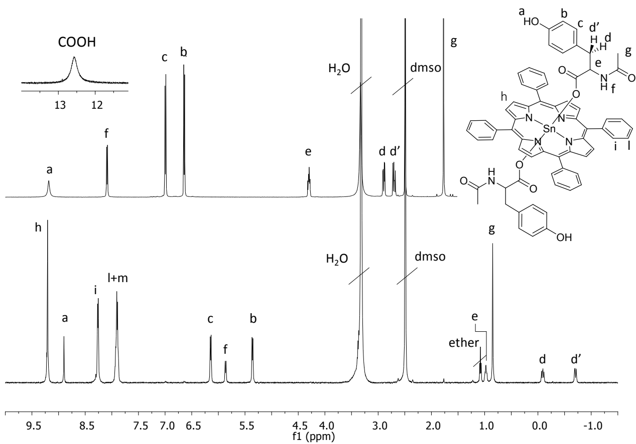
Figure S1. 1 H NMR spectra (dmsO- d 6 ) of N-acetyl-L-tyrosine (top) and 1 (bottom).
