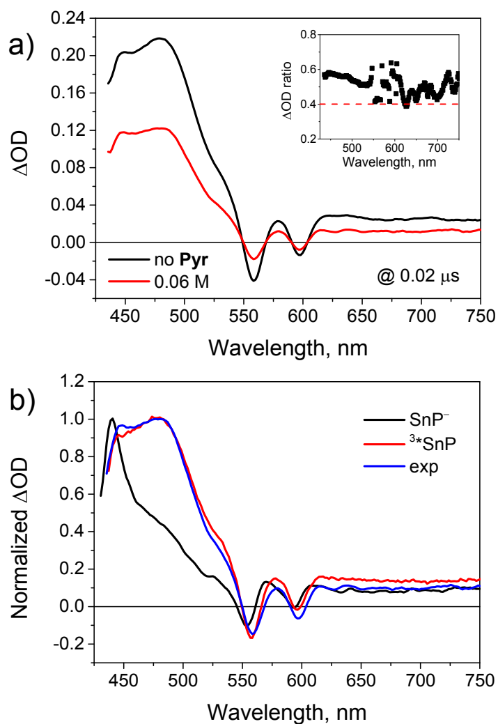
Figure S18. a) Comparison between the prompt transient spectra (0.02 μs time delay) obtained by laser flash photolysis (excitation at 532 nm) of 1 in dichloromethane in the absence (black trace) and presence of 0.06 M pyrrolidine (red trace), the ratio between the two spectra is depicted in the inset; b) comparison of the normalized differential spectra of the SnP radical anion (obtained by laser flash photolysis of 2 in a 95/5 tetrahydrofuran/water mixture in the presence of 10 mM ascorbic acid), of the SnP triplet excited state (obtained by flash photolysis of 2 , Figure S13), and the prompt spectrum (0.02 μs time-delay) obtained by flash photolysis of 1 in dichloromethane with 0.06 M pyrrolidine.
