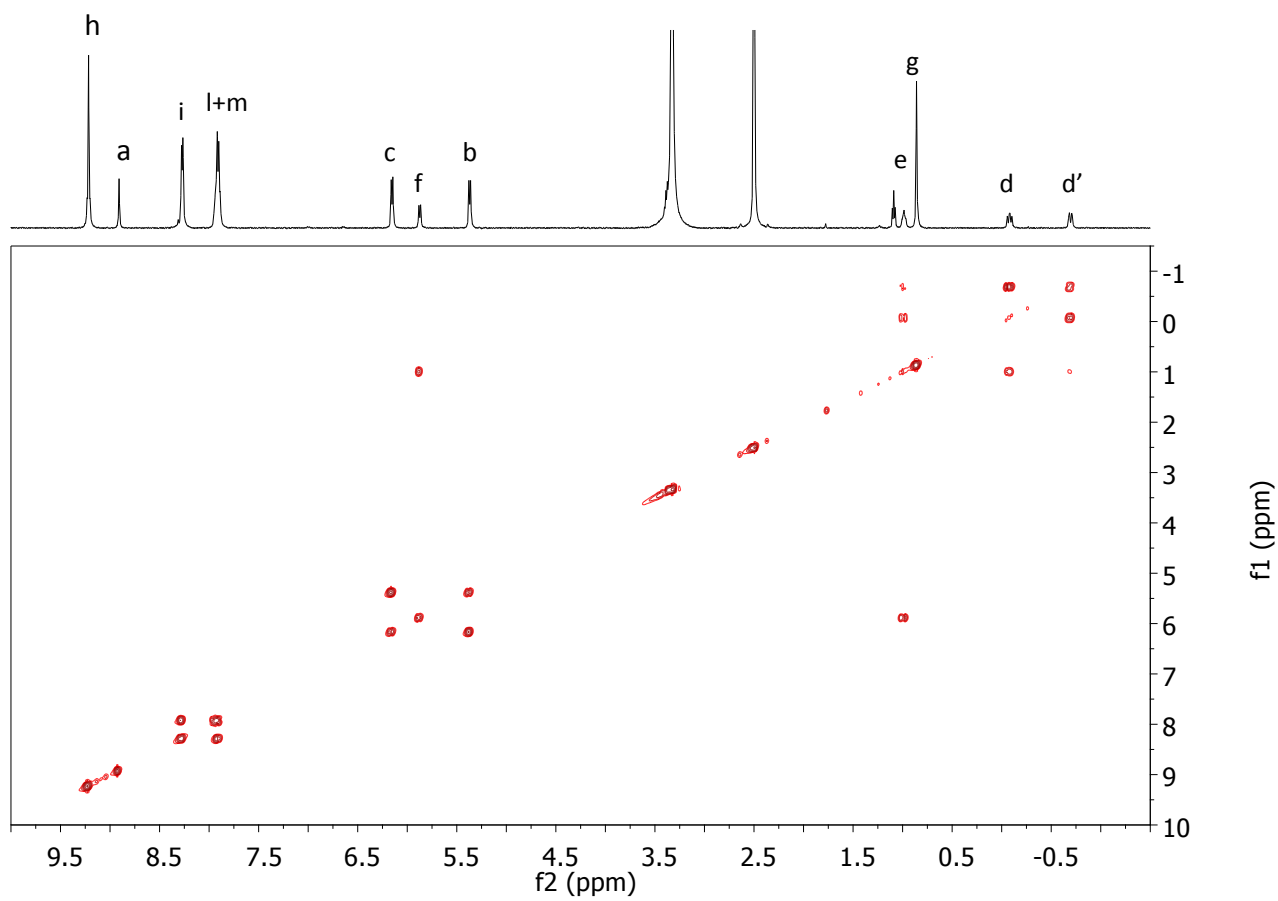
Figure S2. H-H COSY spectrum (dms0- d 6 ) of 1 .
