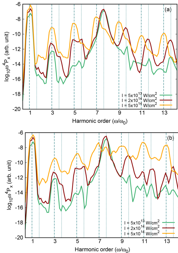
Figure 12. HHG spectra in the dipole form at the equilibrium internuclear distance of R = 2.0 au up to the 13th harmonic with laser intensities I = 5 \times 10^{13} \text{ W/cm}^2 , I = 2 \times 10^{14} \text{ W/cm}^2 , and I = 5 \times 10^{14} \text{ W/cm}^2 for (a) grid and (b) Gaussian basis sets. For each HHG spectrum, the dashed line indicates the position of the harmonics, and the dotted line indicates the hyper-Raman lines at position \tilde{\omega} \pm 2k\omega_0 67 where k is an integer and \tilde{\omega} = 7.65\omega_0 is the resonance of the first excited state.
