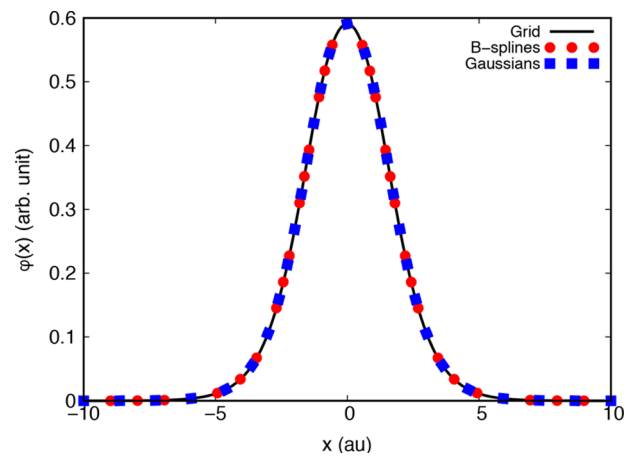
Figure 1. Ground-state wave function of H_2^+ (at the equilibrium internuclear distance of R = 2.0 au) calculated using grid, B-spline, and Gaussian basis.
