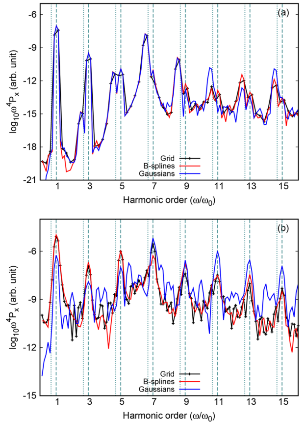
Figure 6. HHG spectra calculated from the electron dipole at the equilibrium internuclear distance R = 2.0 au up to the 15th harmonic with laser intensities (a) I = 10^{14} W/cm ^2 and (b) I = 5 \times 10^{14} W/cm ^2 . The dashed lines indicate the position of the harmonics while the dotted lines indicate the hyper-Raman lines at position \tilde{\omega} \pm 2k\omega_0 67 where k is an integer and \tilde{\omega} = 6.69\omega_0 is the resonance with the first excited state.
