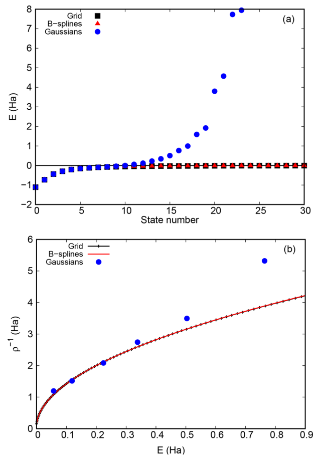
Figure 2. (a) Eigenvalues of H_2^+ up to the 30th eigenstate. (b) Inverse of the normalized density of continuum states.
