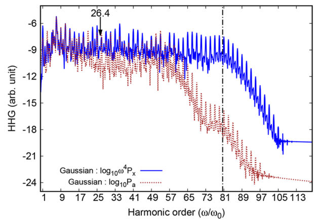
Figure 5. HHG spectra calculated from the electron dipole and the electron acceleration at the equilibrium internuclear distance of R = 2.0 au with a laser intensity of I = 5 \times 10^{14} W/cm ^2 using Gaussian basis sets. The dot-dashed line is the cutoff energy E_{\text{cutoff}} = 80.5\omega_0 and the arrow points to the expected position of the two-center interference minimum, extracted from the recombination dipole which is identical to the one extracted from the recombination acceleration.
