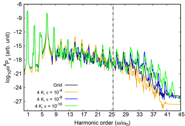
Figure 9. HHG spectra from the dipole at the equilibrium internuclear distance R = 2.0 au with I = 5 \times 10^{13} W/cm 2 obtained with the grid and with the Gaussian basis sets with linear-dependency thresholds \varepsilon = 10^{-4} , \varepsilon = 10^{-8} , and \varepsilon = 10^{-10} .
