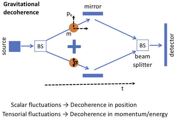
FIG. 1. A quantum system moving in a stochastic gravitational background decoheres. If the scalar component of the metric dominates, then decoherence occurs in position. If the tensorial components dominate then decoherence occurs in momentum and/or energy. Decoherence can be detected by matter-wave interferometers, for example, atom interferometers. A wave packet is split in two parts traveling along different paths, before they recombine by a detector measuring the interference. The relevant parameters are the time of flight t and the transverse momentum p_k .
