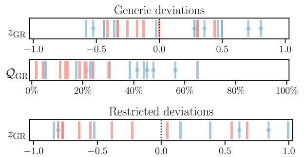
FIG. 8. Figures of merit for the GWTC-2 parametrized tests results. Each vertical stripe corresponds to a given \delta\hat{\varphi}_i as estimated using IMRPHENOMPV2 (blue) or SEOBNRV4_ROM (red); circles identify the postmerger coefficients \{\delta\hat{\alpha}_i, \delta\hat{\beta}_i\} . The top two strips summarize the hierarchical results for generic deviations across events: the z -score for \delta\hat{\varphi}_i = 0 , z_{GR} , and the two-dimensional quantile for the hyperparameters \mu = \sigma = 0 , Q_{GR} . The bottom strip shows an equivalent z -score obtained by restricting to identical deviations across events. The generic (restricted) z -scores correspond to the filled (unfilled) distributions in Fig. 6, and Q_{GR} to those in Fig. 7.
