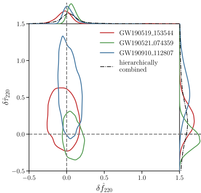
FIG. 14. The 90% credible region of the joint posterior distribution of the fractional deviations of the frequency \delta \hat{f}_{220} and the damping time \delta \hat{\tau}_{220} , and their marginalized posterior distributions, for the \ell = |m| = 2, n = 0 mode from the PSEOBNRV4HM analysis. We only include events that have \text{SNR} > 8 in both the inspiral and postinspiral stage in this plot where we have sufficient information to break the degeneracy between the binary total mass and the fractional deviation parameters in the absence of measurable HMs. The measurements of the fractional deviations for individual events, and as a set of measurements, both show consistency with GR.
