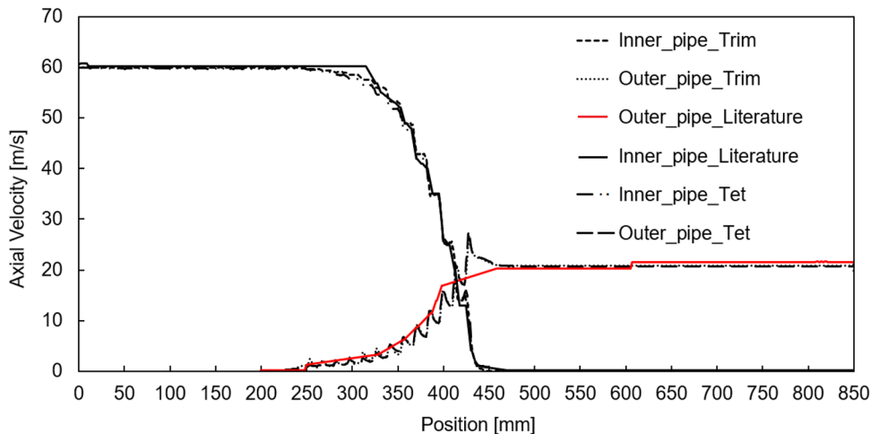
Fig. 5 Comparison between axial velocities. Real geometry model
