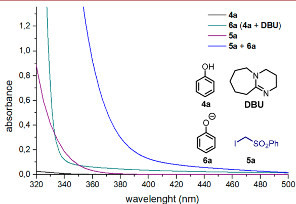
Figure 2. Optical absorption spectra acquired in acetonitrile in 1 mm path quartz cuvettes: [4a] = 1.5 M; [5a] = 0.5 M; [DBU] = 1.5 M. DBU: 1,8-diazabicyclo[5.4.0]undec-7-ene.
