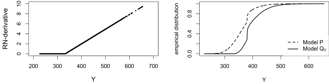
Fig. 1. Left: Radon-Nikodym derivative of Q_Y against Y . Right: Stressed probability distributions of Y under models P , Q_Y .
