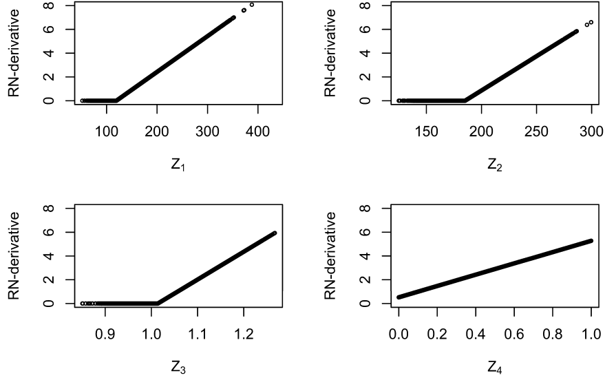
Fig. 3. Radon-Nikodym derivatives of stressed models Q_{Z_i} for i = 1, \dots, 4 .
