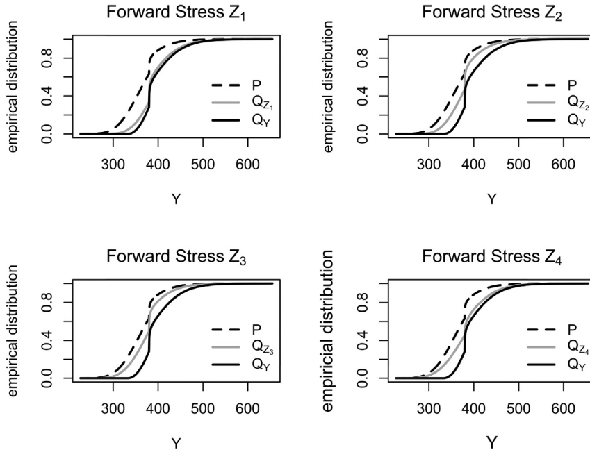
Fig. 4. Stressed probability distributions of Y under the baseline model P and the stressed models Q_Y and Q_{Z_i} for i = 1, \dots, 4 .
