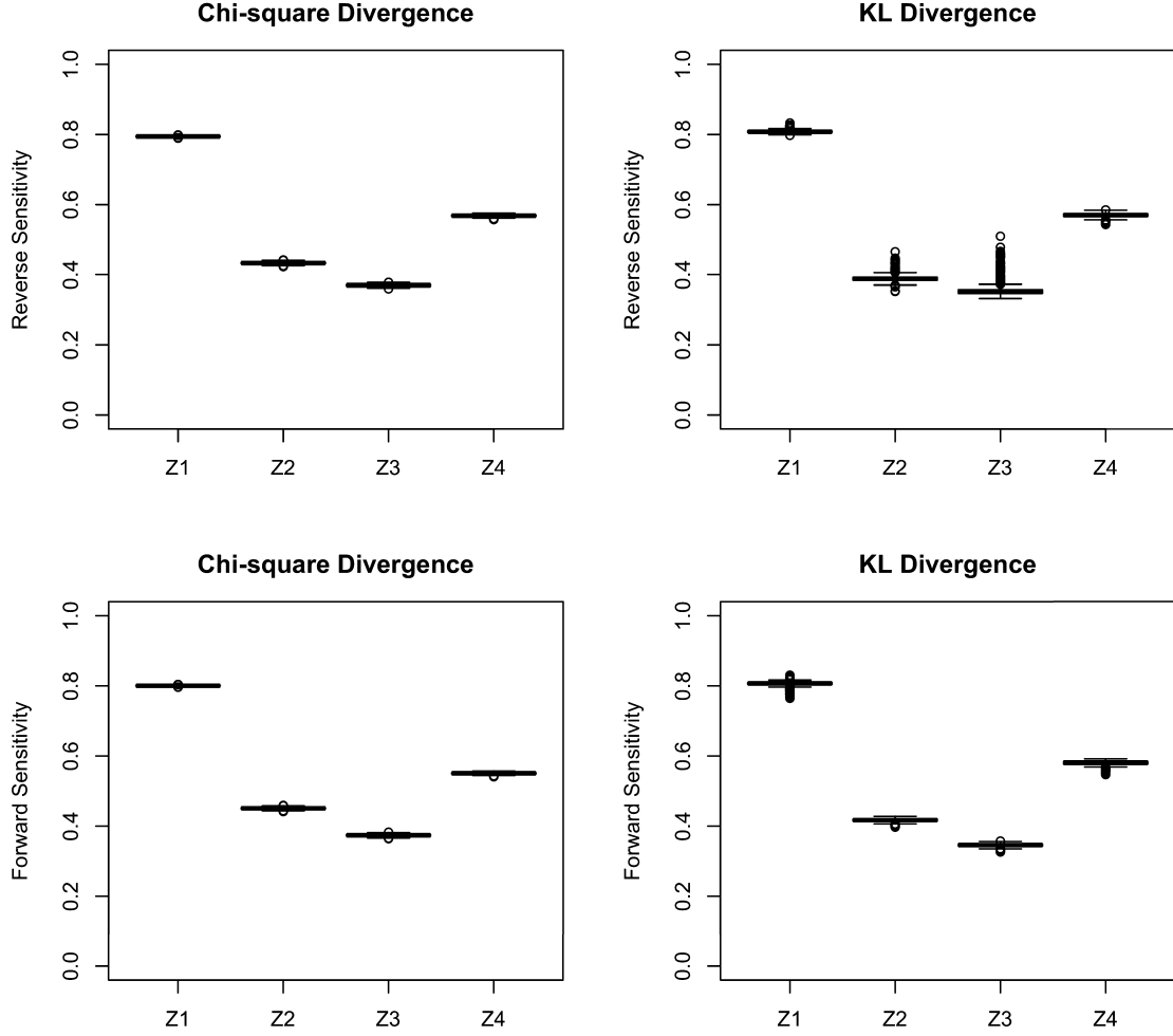
Fig. 5. Box plots of reverse and forward sensitivities of input factors under \chi^2 - and Kullback-Leibler divergences, for m = 1000 sets of n = 10^5 simulated scenarios.
