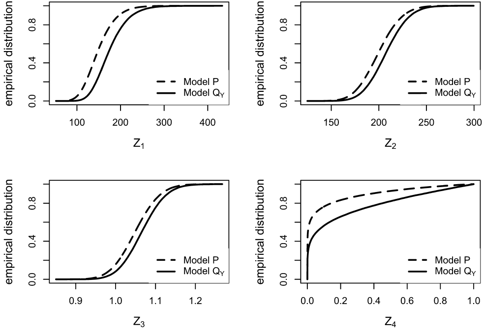
Fig. 2. Empirical distributions of the input factors under the baseline and stressed models P , Q_Y .
