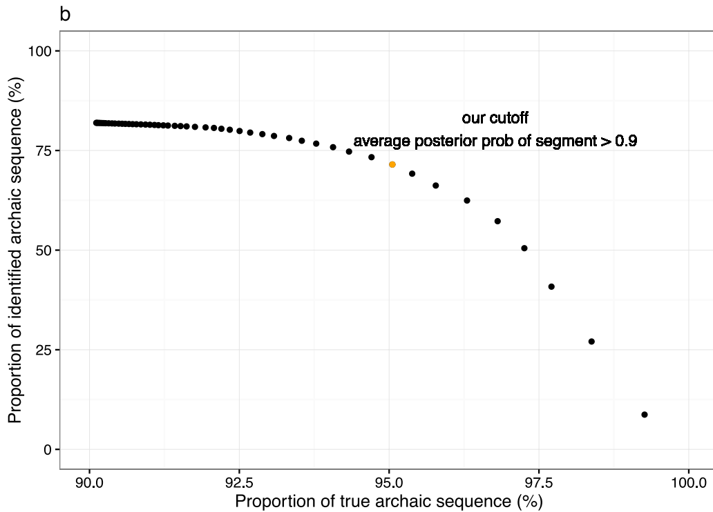
Extended Data Fig. 1 | Estimates of the false-positive rate of archaic inference based on simulations. a, Length distributions of false-positive and true-positive calls for fragments inferred to be archaic, and the length distributions for simulated archaic fragments that were found and those that
