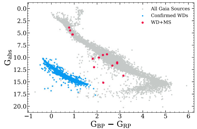
Figure 9. A Gaia HR diagram showing all spectroscopically confirmed white dwarfs within 40 pc as blue points, alongside all other Gaia sources in the same volume which have \text{parallax\_over\_error} > 1 and \text{astrometric\_excess\_noise} < 1.5 from Gaia DR3 as grey points. White dwarfs in unresolved binaries with main-sequence companions that are not in the Gentile Fusillo et al. (2021) catalogue are shown as larger red points.
