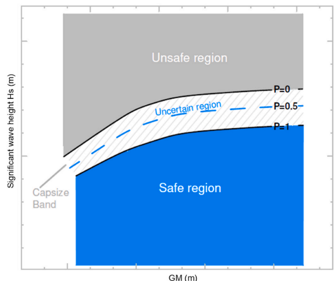
Fig. 1. Capsize band for one damage scenario and different loading conditions and sea states.
