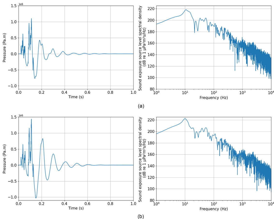
FIG. 2. Source waveforms (left panels) and sound exposure source level spectral density (right panels) simulated with AASM for (a) 8867 in. 3 and (b) 11 441 in. 3 configurations at a bearing of 54.25° resulting from the difference between the towing direction (237.25°) and the direction of propagation towards the NEMO-SN1 observatory (291.5°).
