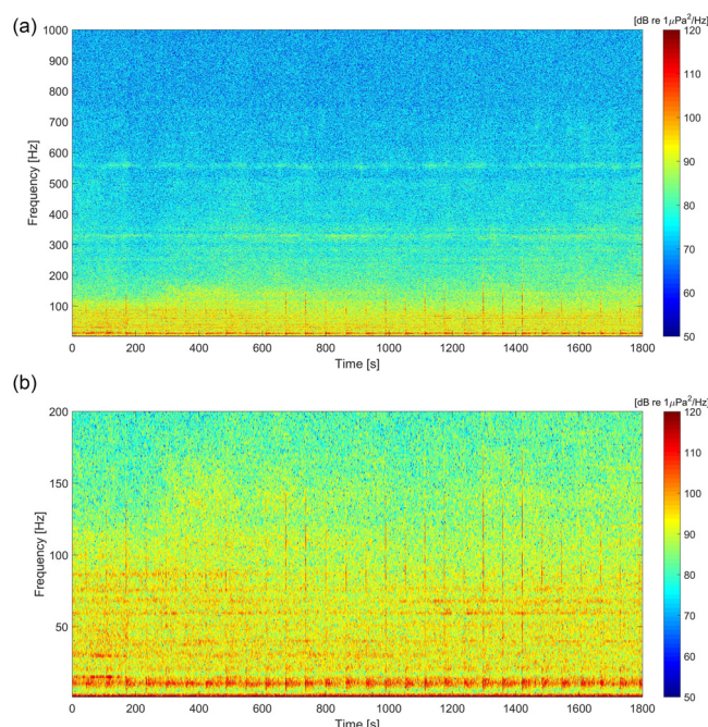
FIG. 4. Spectrograms of acoustic recordings with airgun pulses at NEMO-SN1 computed with 2048-point fast Fourier transform, Hanning window, and 98% overlap (30-min recording from 16:40 to 17:10 UTC on November 6, 2012). (a) Full-scale version of the spectrogram up to 1 kHz; (b) zoomed-in version of the spectrogram up to 200 Hz.
