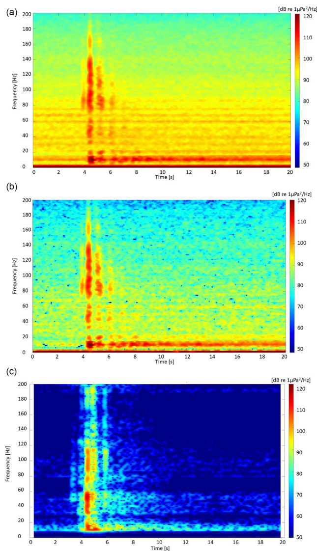
FIG. 7. Panels showing three spectrograms for the 8867 in. 3 configuration: (a) average of the pulses recorded at NEMO-SN1 without denoising, (b) pulses recorded at NEMO-SN1 with the application of denoising, (c) spectrogram of the simulated signal.
