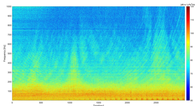
FIG. 5. Typical situation of marine traffic recorded at NEMO-SN1 (Viola et al. , 2017). The spectrogram was computed with 4096-point fast Fourier transform, Hanning window, 0.1 s temporal resolution, 0.48 Hz frequency resolution.
