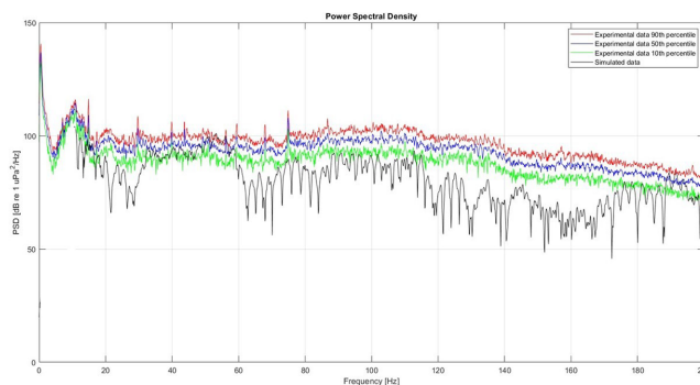
FIG. 8. Comparison between the spectral densities of the simulated and recorded signals at a distance of 650 km from the source. PSD plot of the recorded signal averaged over a time window of 30 min.
