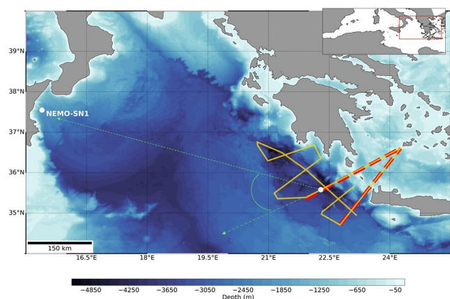
FIG. 1. Map of the study area showing the location of the NEMO-SN1 observatory (Latitude 37.5477° N, Longitude 15.3975° E) and the ULYSSE survey (Laigle and Sachpazi, 2012). The yellow lines indicate the reflection survey and the orange dashed lines the refraction survey. The unlabeled white dot shows the location of the source. The green dotted lines represent the ship heading and the bearing (54.25°) used in the simulations. The track data for the ship route was downloaded from SISMER IFREMER ( https://donnees-campagnes.flotteoceanographique.fr/search;?201203010055.nvi file).
