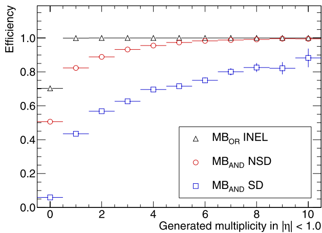
Fig. 2 Charged-particle multiplicity dependence of the selection efficiency, for INEL events ( triangles ) with MB_{OR} selection, and for NSD ( circles ) and SD ( squares ) events with MB_{AND} selection obtained with a simulation of the 0.9 TeV data
