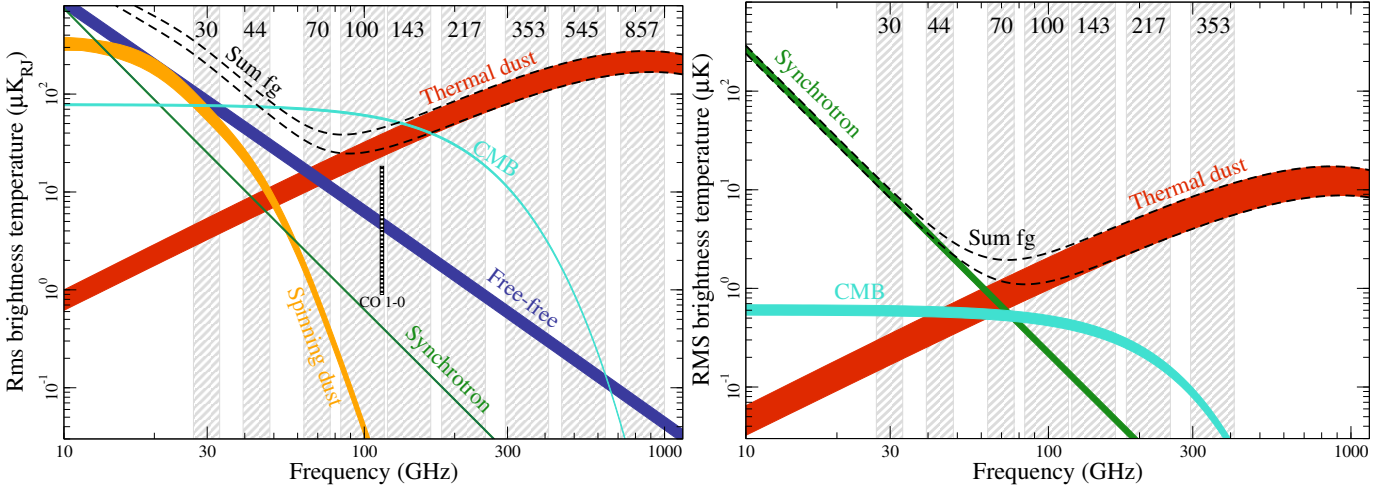
Fig. 18. Brightness temperature rms of the high-latitude sky as a function of frequency and astrophysical component for temperature (left) and polarization (right). For temperature, each component is smoothed to an angular resolution of 1^\circ FWHM, and the lower and upper edges of each line are defined by masks covering 81 and 93% of the sky, respectively. For polarization, the corresponding smoothing scale is 40' , and the sky fractions are 73 and 93%.
