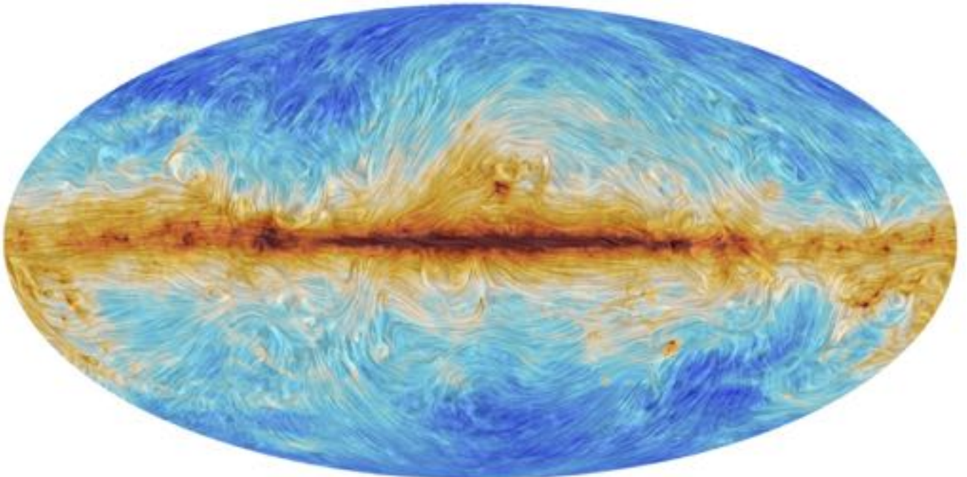
Fig. 24. All-sky view of the angle of polarization at 353 GHz, rotated by 90^\circ to indicate the direction of the Galactic magnetic field projected on the plane of the sky. The colours represent intensity, dominated at this frequency by thermal dust emission. The “drapery” pattern was obtained by applying the line integral convolution (LIC; Cabral & Leedom 1993) using an IDL implementation provided by Diego Falceta-Goncalves ( http://each.uspnet.usp.br/fgoncalves/pros/lic.pro ). Where the field varies significantly along the line of sight, the orientation pattern is irregular and difficult to interpret.
