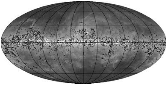
Fig. 15. All-sky distribution of the 13 188 PGCC Galactic cold clumps (black dots) and the 54 cold sources (grey dots) located in the Large and Small Magellanic Clouds. The background map is the 857 GHz Planck band, shown in logarithmic scale from 10^{-2} to 10^2 MJy sr ^{-1} .
