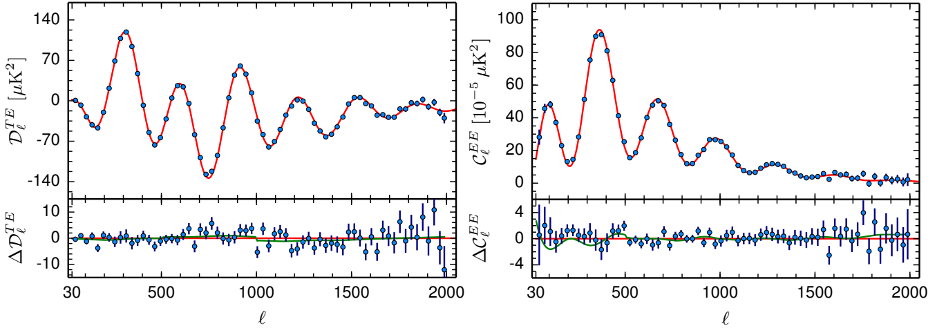
Fig. 12. Frequency-averaged TE (left) and EE (right) spectra (without fitting for T - P leakage). The theoretical TE and EE spectra plotted in the upper panel of each plot are computed from the best-fit model of Fig. 11. Residuals with respect to this theoretical model are shown in the lower panel in each plot. The error bars show \pm 1 \sigma errors. The green lines in the lower panels show the best-fit temperature-to-polarization leakage model, fitted separately to the TE and EE spectra. From Planck Collaboration XIII (2015) .
