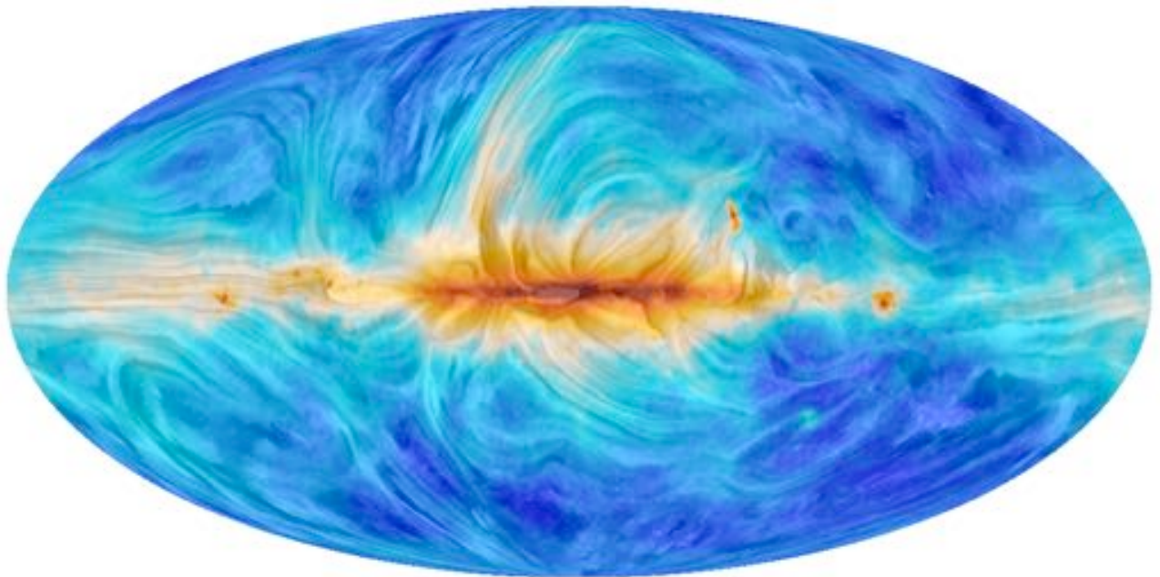
Fig. 22. All-sky view of the angle of polarization at 30 GHz, rotated by 90^\circ to indicate the direction of the Galactic magnetic field projected on the plane of the sky. The colours represent intensity, dominated at this frequency by synchrotron emission. The “drapery” pattern was obtained by applying the line integral convolution (LIC; Cabral & Leedom 1993) using an IDL implementation provided by Diego Falceta-Goncalves ( http://each.uspnet.usp.br/fgoncalves/pros/lic.pro ). Where the field varies significantly along the line of sight, the orientation pattern is irregular and difficult to interpret.
