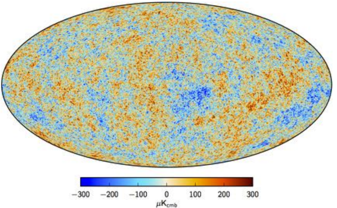
Fig. 9. Maximum posterior CMB intensity map at 5' resolution derived from the joint baseline analysis of Planck , WMAP, and 408 MHz observations. A small strip of the Galactic plane, 1.6% of the sky, is filled in by a constrained realization that has the same statistical properties as the rest of the sky.
