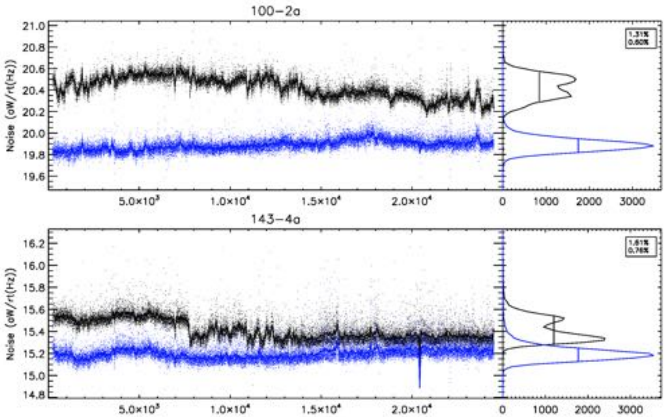
Fig. 1. Noise stationarity for a selection of two bolometers. The left panels show the total noise trends for each bolometer (dots). The solid line shows a running box average. The black dots are from the 2013 data release and the blue dots concern this release. The right panels show a histogram of the trends on the left. The box gives the width of the distribution at half maximum, as measured on the histogram, normalized to the mean noise level. The time response deconvolution has changed between the two data release and hence the absolute noise level is different.
