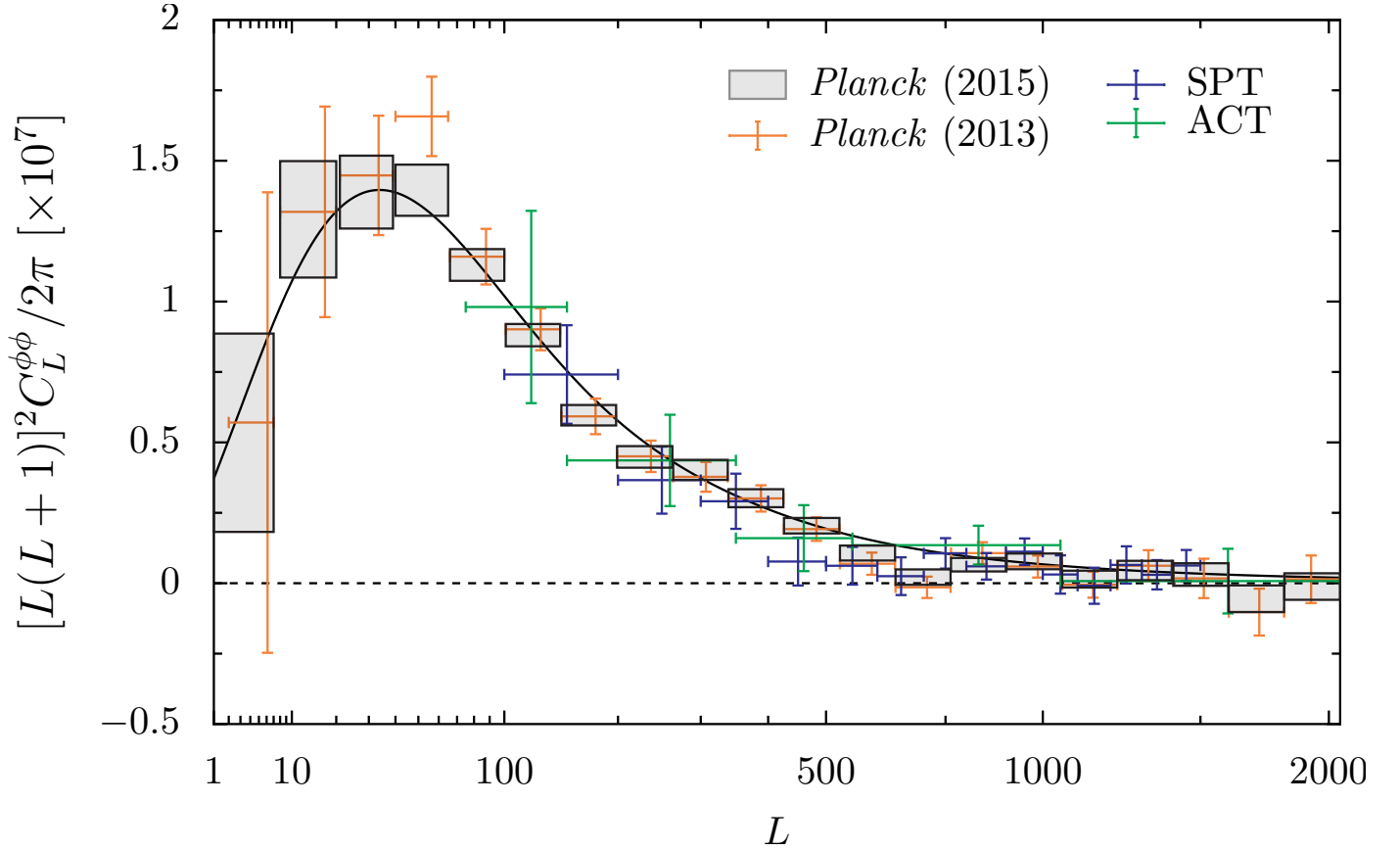
Fig. 20. Lensing potential power spectrum estimate from the 2015 data release (Planck Collaboration XV 2015), based on the SMICA CMB map, as well as previous reconstructions from Planck as well as other experiments for comparison.
