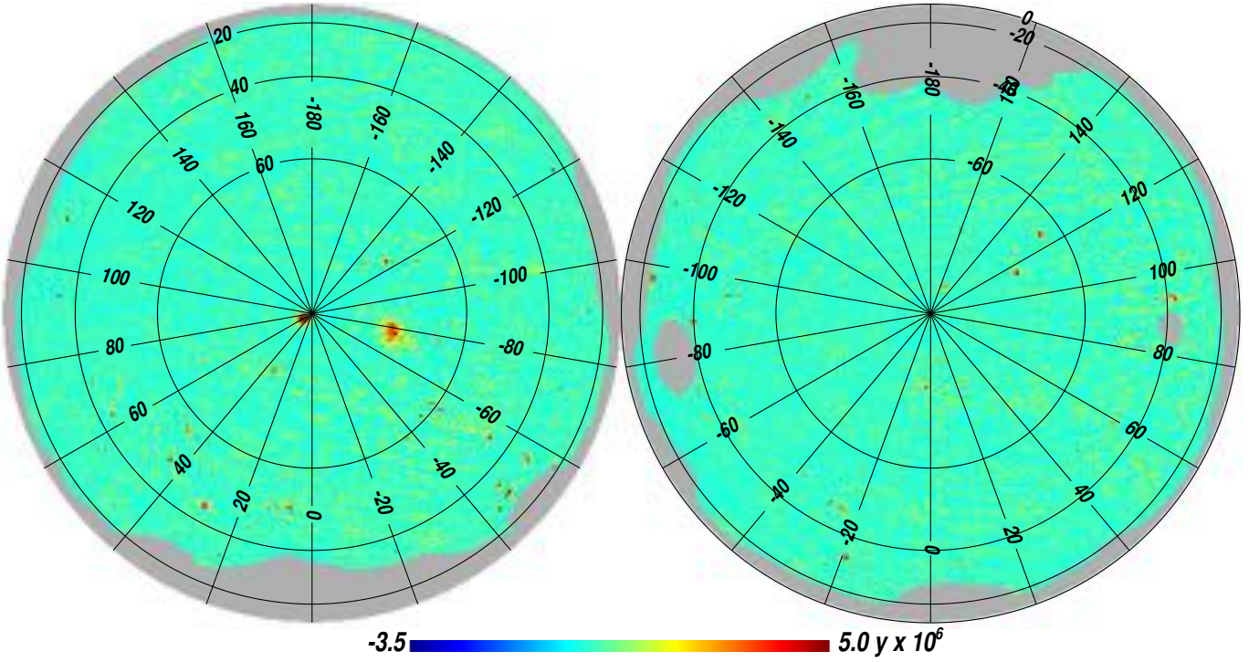
Fig. 19. Orthographic projection of the reconstructed Planck all-sky y -map in Compton parameter units (Planck Collaboration XXII 2015). For illustration purposes and to enhance the tSZ signal-to-noise ratio, the y -map has been Wiener filtered. Positive sources in the map correspond to clusters and super-clusters of galaxies with strong tSZ emission. In particular, the Coma and Virgo clusters are clearly visible near the north Galactic pole. The region of strongest contamination from Galactic foreground emission in the Galactic plane has been partially masked.
