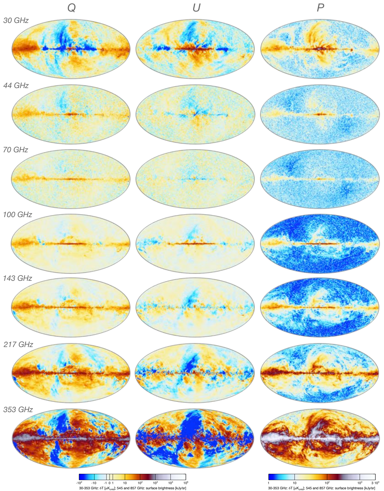
Fig. 8. The seven Planck polarization maps between 30 and 353 GHz, shown in Stokes Q and U , as well as in total polarized intensity ( P ). The LFI maps are not bandpass-corrected; the HFI maps are. The color scale uses the same function as in Fig. 7, but the range limits have been adjusted.
