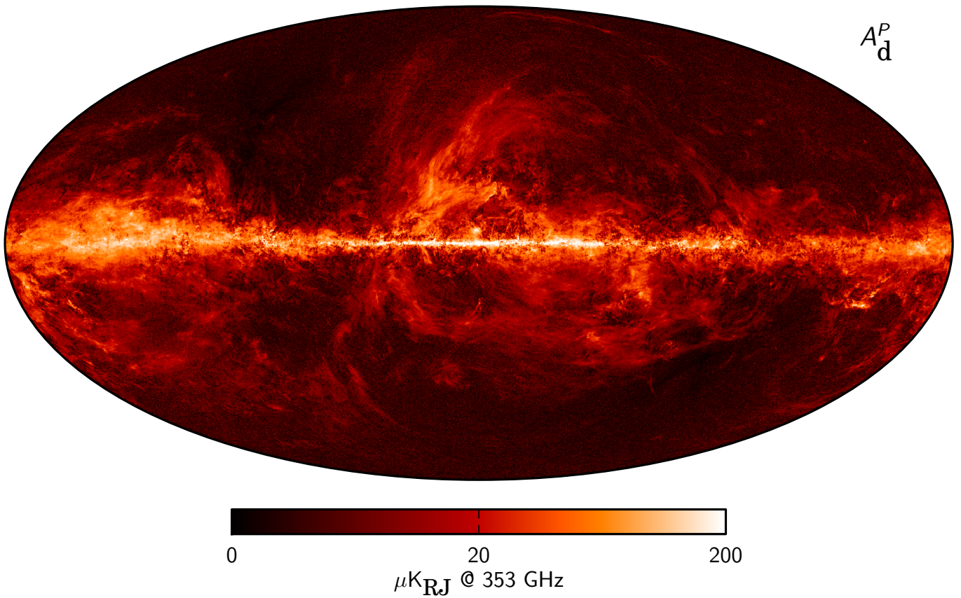
Fig. 23. Dust polarization amplitude map, P = \sqrt{Q^2 + U^2} , at 353 GHz, smoothed to an angular resolution of 10' , produced by the diffuse component separation process described in (Planck Collaboration X 2015) using Planck and WMAP data.
