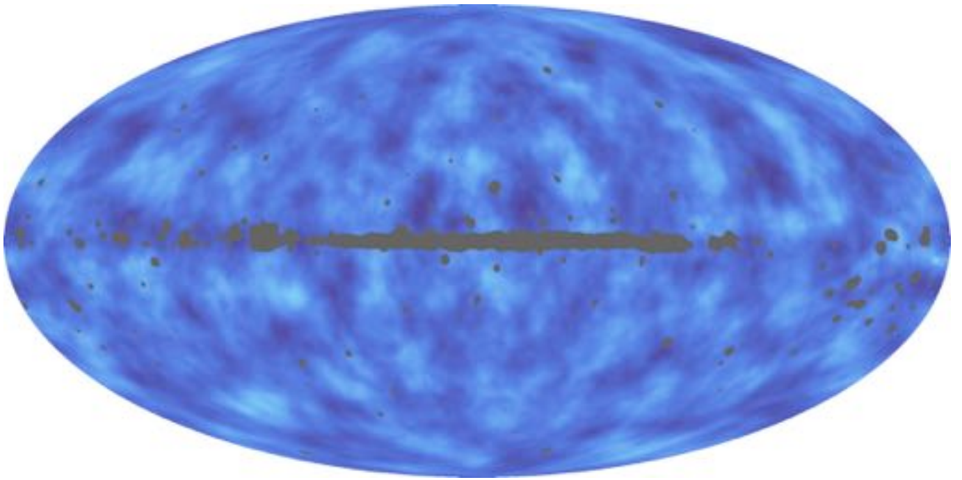
Fig. 13. Wiener-filtered lensing potential estimate with minimal masking (using the NILC component separated map), in Galactic coordinates with a Mollweide projection (Planck Collaboration XV 2015). The reconstruction has been bandlimited to 8 \leq L \leq 2048 (where, following convention, L is used as the multipole index in the lensing power spectrum).
