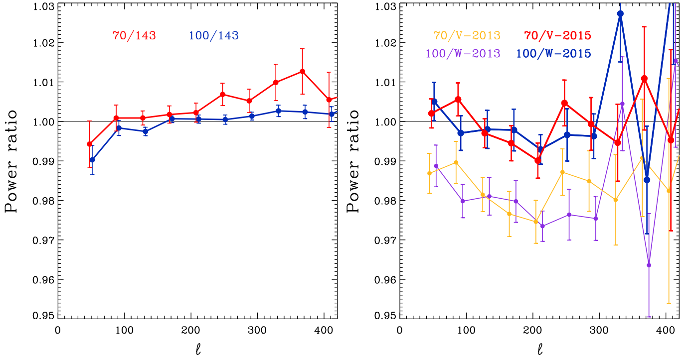
Fig. 6. Ratios of power spectra over the region of the first acoustic peak, uncorrected for foregrounds (which vary over the three frequencies), over 60 % of the sky. The uncertainties are the errors on the mean within each \Delta\ell = 40 bin of the ratios computed \ell by \ell . Left: Ratios of 70 and 100 GHz TT spectra to 143 GHz. The low values at \ell = 50 are due to diffuse foregrounds at 143 GHz. The rise to higher multipoles in the 70/143 ratio is due to discrete foregrounds. Right: Ratio of TT spectra of Planck 70 and 100 GHz to WMAP V and W bands, as calculated for Planck 2013 data ( Planck Collaboration XXXI 2014 ) and for the 2015 data. The near-overlap of frequencies between the Planck and WMAP bands means that foregrounds have no appreciable effect on the ratios. The effect of the calibration changes in Planck between 2013 and 2015 that are discussed in this paper is clear. There is now excellent agreement within statistical errors between Planck and WMAP in the region of the spectrum where both have high S/N.
