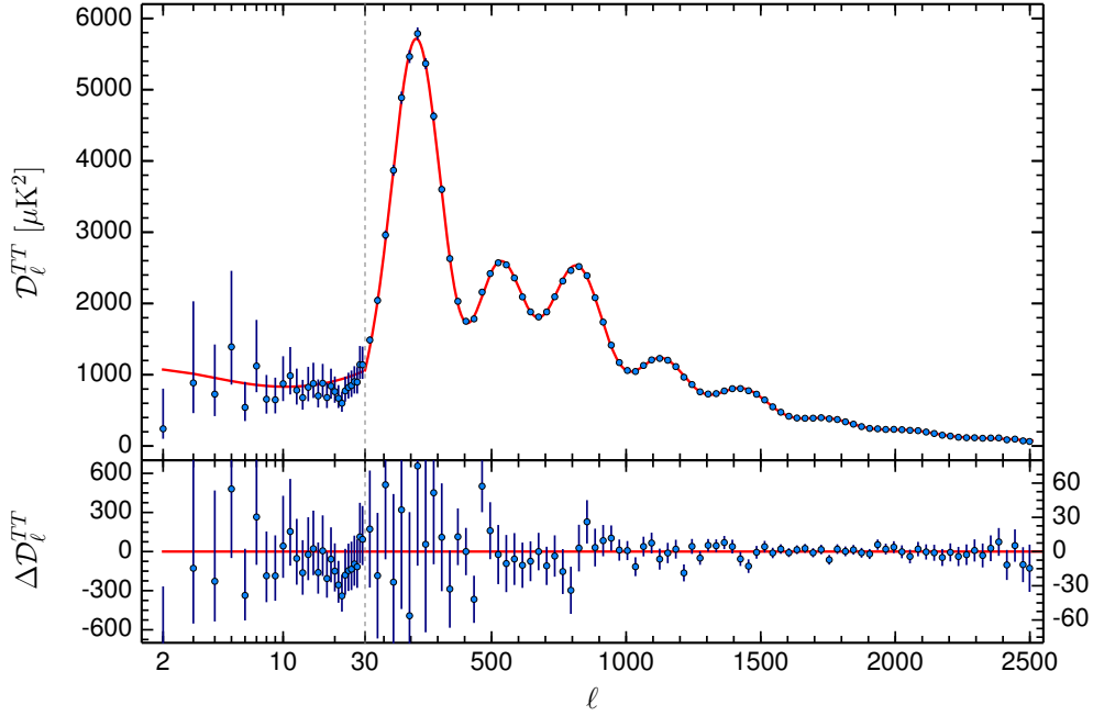
Fig. 11. The Planck 2015 temperature power spectrum. At multipoles \ell \geq 30 we show the maximum likelihood frequency-averaged temperature spectrum computed from the cross-half-mission likelihood with foreground and other nuisance parameters determined from the MCMC analysis of the base \Lambda CDM cosmology. In the multipole range 2 \leq \ell \leq 29 , we plot the power spectrum estimates from the Commander component-separation algorithm computed over 94 % of the sky. The best-fit base \Lambda CDM theoretical spectrum fitted to the PlanckTT+lowP likelihood is plotted in the upper panel. Residuals with respect to this model are shown in the lower panel. The error bars show \pm 1 \sigma uncertainties. From Planck Collaboration XIII (2015) .
