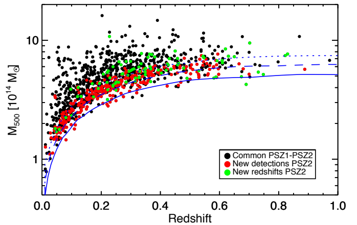
Fig. 14. Distribution of the 1093 PSZ2 clusters with counterparts with known redshift in the M_{500}-z plane. New PSZ2-detected clusters are indicated with red dots, while common PSZ1 and PSZ2 clusters are indicated by black dots. Green dots mark the common PSZ2–PSZ1 detections where we have updated the redshift value for the PSZ2. The solid, dashed, and dotted lines indicate the limiting mass at 20 %, 50 %, and 80 % survey completeness, respectively.
