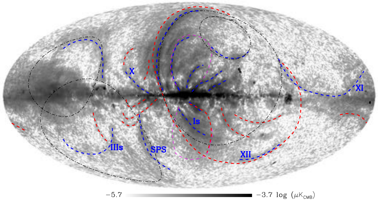
Fig. 21. Synchrotron polarization amplitude map, P = \sqrt{Q^2 + U^2} , at 30 GHz, smoothed to an angular resolution of 60' , produced by a weighted sum of Planck and WMAP data as described in (Planck Collaboration XXV 2015). The traditional locii of radio loops I–IV are marked in black, a selection of the spurs identified by Vidal et al. (2014) in blue, the outline of the Fermi bubbles in magenta, and features discussed for the first time in (Planck Collaboration XXV 2015) in red. Our measured outline for Loop I departs substantially from the traditional small circle.
