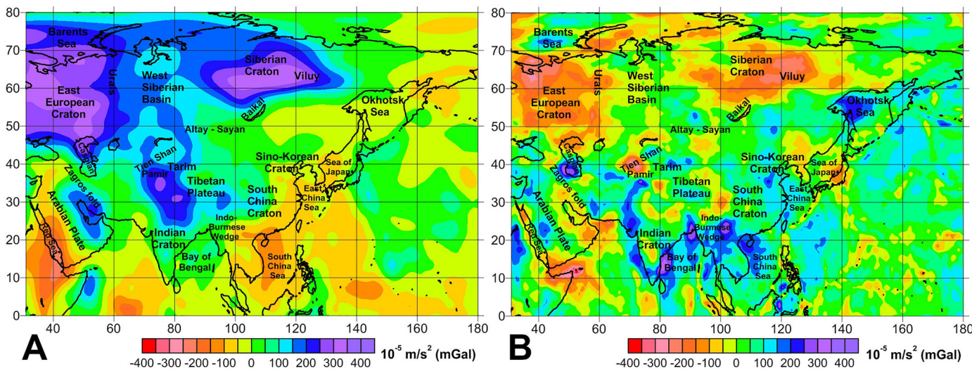
Figure 6. (a) Gravity effect of the initial thermal model of the mantle and (b) residual gravity anomalies obtained by removing this effect from the total mantle gravity field shown in Figure 4a.
