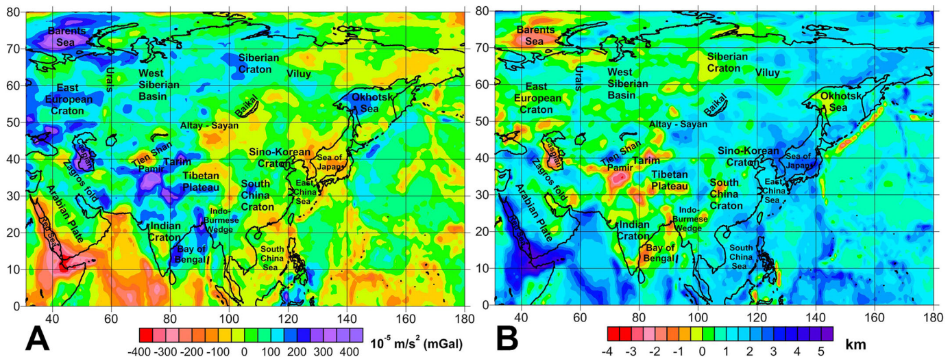
Figure 4. (a) Mantle gravity anomalies and (b) residual topography obtained by removing the crustal effects from the observed fields. The density of the residual topography is 2670 \text{ kg/m}^3 .
