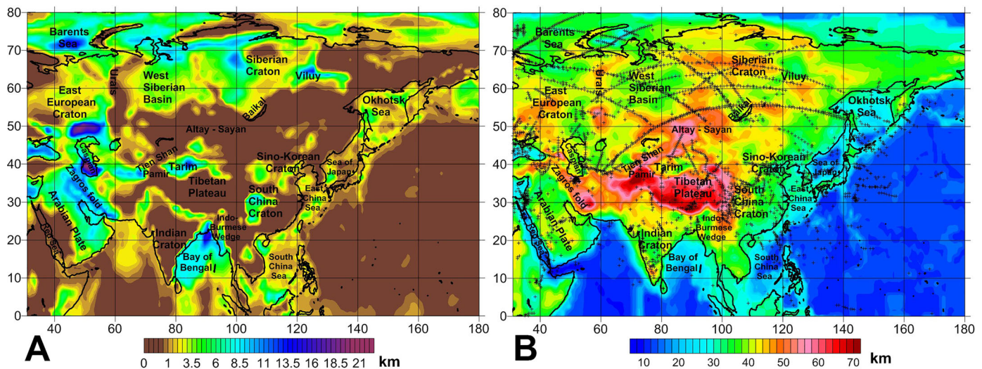
Figure 2. (a) Thickness of sediments in the study region. (b) Depth to the Moho from sea level. Crosses show seismic determinations used for construction of the crustal model.
