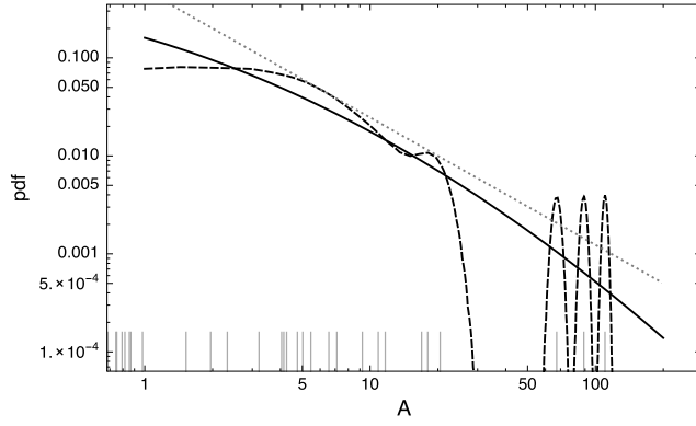
Fig. 3. Pdf of the values of A in the case of the aggregated tumour spheroid data (spheroids from the 9 L, MR1 and Rat-T1 cell lines): the original data points are shown as a “rug plot” (the positions marked by the vertical bars in the lower part of the plot). In addition to the glucose uptake values given in [13] we have used \eta = 6.5 \times 10^{-12} and \lambda = 93.9 \mu\text{m} for 9 L spheroids, \eta = 4.2 \times 10^{-12} and \lambda = 123.6 \mu\text{m} for Rat-T1 spheroids; \eta = 8.9 \times 10^{-12} and \lambda = 91.0 \mu\text{m} for MR1 spheroids. The solid curve is the lognormal fit, the dashed line is the empirical smoothed kernel density, and the dotted line is a power-law with exponent -1.3 .
