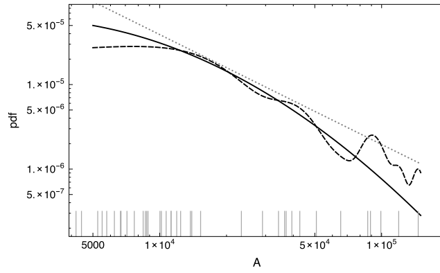
Fig. 4. Pdf of the values of A in the case of human solid tumours: the original data points are shown as a “rug plot” (the positions marked by the vertical bars in the lower part of the plot). In addition to the glucose uptake values given in [13] we have used \eta = 3.7 \times 10^{-12} and \lambda = 99.4 \mu\text{m} . The solid curve is the lognormal fit, the dashed line is the empirical smoothed kernel density, and the dotted line is a power-law with exponent -1.3 .
