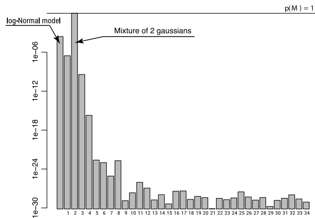
Fig. 6. Ranking of hypotheses in the case of solid tumours in vivo . The numbers on the x axis mean the number of mixture components, the y axis is the value of the marginal likelihood.
