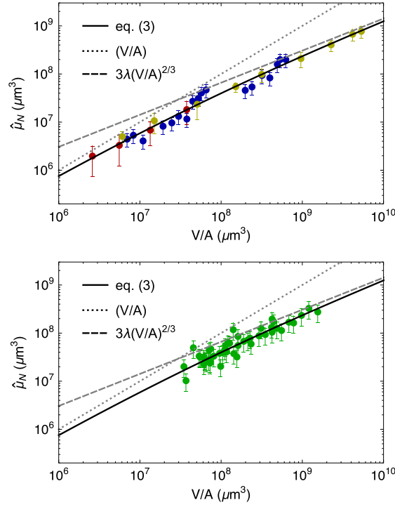
Fig. 1. Metabolic rate data \hat{\mu}_N = \mu/\eta A^{1/3} vs. V/A ( \mu\text{m}^3 ). The figure shows a breakdown of the data originally presented in [13]. Upper panel: tumour spheroids cultured in vitro using different cell lines. Lower panel: data from human tumours, that include breast, uterine and ovarian carcinomas, melanomas, thyroid carcinomas, colon and lung carcinomas. All of these human tumours correspond presumably to different cell-specific metabolic rates \eta . The dotted line is \hat{\mu}_N = V , while the dashed line is \hat{\mu}_N = V^{2/3} , which are the extreme behaviours derived from Eq. (1).
