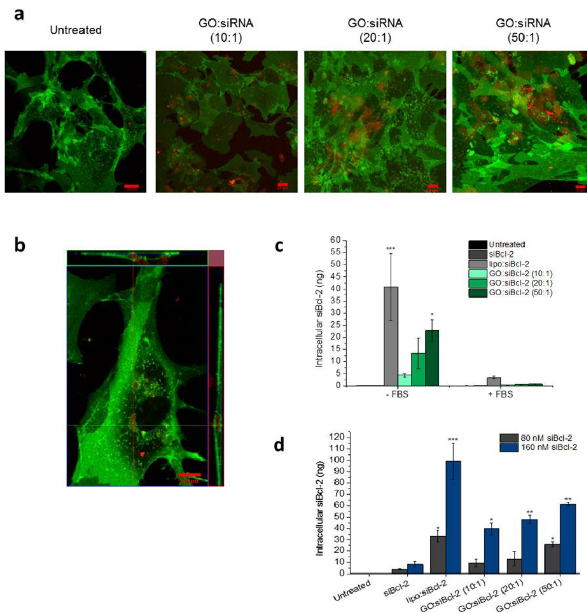
Figure 3. Uptake of GO:siRNA complexes 4 h after exposure. (a) GO uptake in MEFs was visualised by live cell confocal microscopy, 4 h after transfection, thanks to the intrinsic fluorescence of the material. Images represent maximum intensity projection of the fluorescence across the Z-stack, corresponding to plasma membrane staining (green) and GO (red). Scale bars show 10 or 20 \mu\text{m} . (b) Orthogonal view confirms intracellular localisation of the GO, upon exposure to GO:siRNA (50:1). Green signal corresponds to cell membrane staining, red signal corresponds to GO. Scale bar shows 10 \mu\text{m} . (c) Intracellularly delivered siRNA was quantified by stem-loop PCR in the presence or absence
