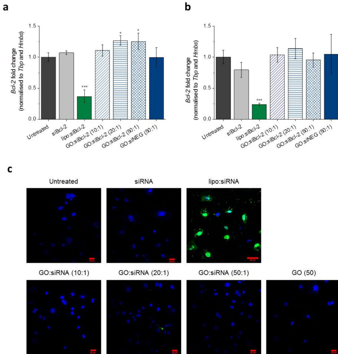
Figure 4. In vitro functional assessment of GO:siRNA complexes. Bcl-2 mRNA expression was studied by RT-qPCR 24 h after transfection with GO:siBcl-2 complexes at (a) [siBcl-2]=80 nM and (b) [siBcl-2]=160 nM. * p < 0.05 and *** p < 0.001 , one-way ANOVA and Tukey post-hoc test, n=3 . (c) siRNA desorption from GO and intracellular trafficking were studied with a RISC-independent, nuclear-targeted and fluorescently-labelled siRNA (siGLO) complexed to GO. 4 h after transfection, siGLO only localised to the nucleus when delivered by a lipid-based transfection reagent. No fluorescence was recovered in any of the GO:siGLO conditions. Green signal corresponds to 6-FAM labelling of siGLO oligonucleotide, blue signal corresponds to Hoechst nuclear staining. Scale bar shows 20 or 50 \mu\text{m} .
