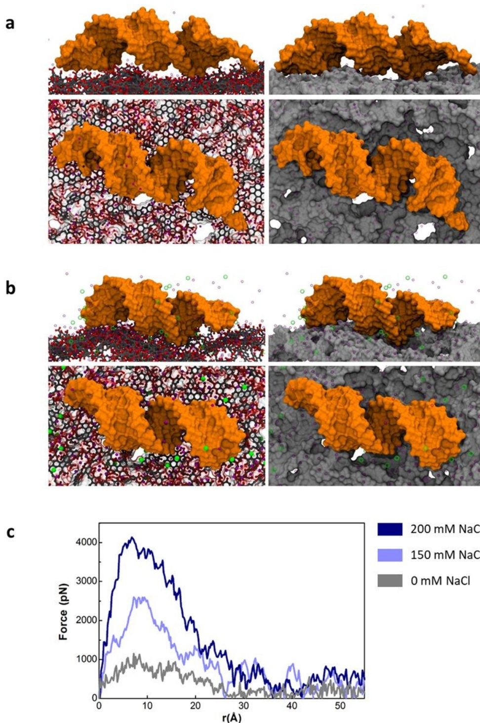
Figure 2. GO:siRNA binding/unbinding by MD simulation. Snapshots extracted from MD calculation of siRNA (represented as an orange shaded surface) in complex with a GO sheet (a) without complementary salts and (b) at 150 mM NaCl ionic strength (top panels, lateral view; bottom panels, top view). Images on the left show the chemical structure of GO explicitly represented with carbon and oxygen atoms colored in grey and red, respectively. In the right panels, we depicted the GO sheet as a grey surface to highlight 3D features. For clarity, water is not shown and Na + and Cl - ions are visualized as purple and green spheres, respectively. (c) SMD simulation of the unbinding process of siRNA from GO. The pulling force as a function of the distance from the center of mass of GO and siRNA in the direction perpendicular to the GO plane is monitored. Color legend: 0 mM, grey; 150 mM, light blue; 200 mM, dark blue.
