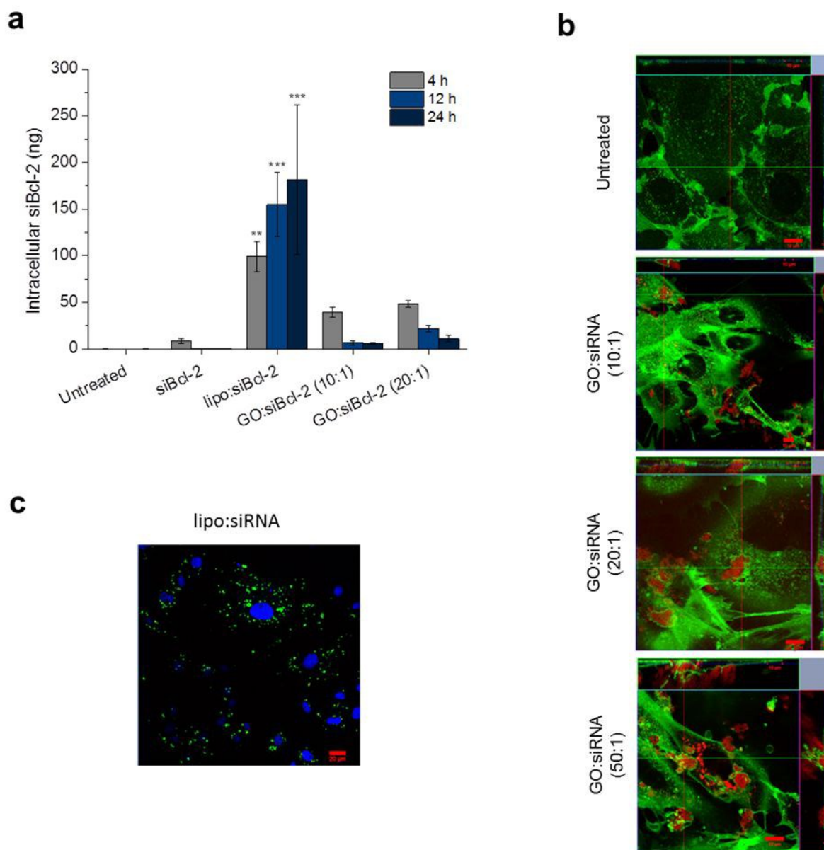
Figure 5. Intracellular fate of GO:siRNA complexes. (a) PCR-based quantification of intracellularly delivered siRNA 4, 12 and 24 h after transfection indicated a sharp decrease of intracellular siRNA between 4 and 12 h time points when delivered by GO:siRNA complexes (** p < 0.01 and *** p < 0.001 , one-way ANOVA and Tukey post-hoc test, n=3 ). (b) 24 h after transfection, GO was still present intracellularly, but sequestered in large vesicles, as shown by live confocal microscopy. Green – Cell Membrane Mask, Red – GO. Scale bars show 10 or 20 \mu\text{m} . (c) Confocal microscopy image of MEFs treated with lipo:siRNA complexes, where siRNA was fluorescently labelled, 24h after transfection. Green – non-coding siRNA-488, Blue – nucleus (Hoechst). Scale bar shows 20 \mu\text{m} .
