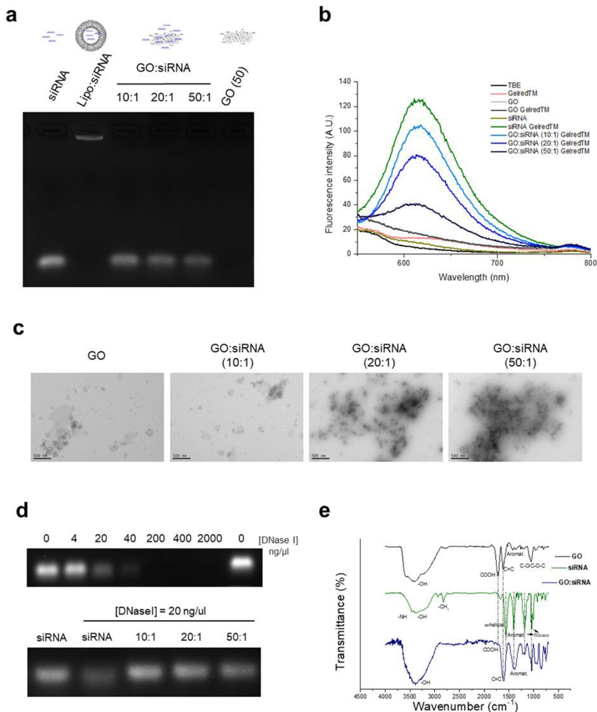
Figure 1. GO:siRNA complexation studies. Complexation of double-stranded siRNA was investigated at 10:1, 20:1 and 50:1 GO:siRNA mass ratios by (a) gel retardation assay, (b) quenching of the fluorescence signal of a nucleic acid dye (Gelred TM ) and (c) transmission electron microscopy (TEM). (d) Exposure to DNase I confirmed complexation, given the absence of siRNA degradation in the presence of GO. (The top gel shows degradation of free siRNA by increasing concentrations of DNase I, the bottom gel shows degradation of free or complexed siRNA at 20 ng/ \mu l DNase I). (e) Differences in ATR-FTIR spectra of GO, siRNA and GO:siRNA (50:1 mass ratio) confirmed the interaction of the oligonucleotide with the GO surface.
