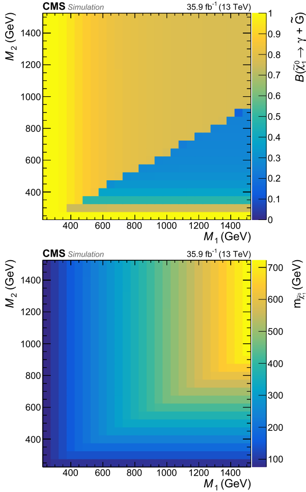
Fig. 2. Branching fractions ( B ) for the NLSP decay to a photon and a gravitino for the GGM scenario (upper). The phase space is spanned by the bino ( M_1 ) and wino ( M_2 ) mass parameters showing the change of the NLSP composition. This change also influences the dependence of the physical mass of the neutralino ( m_{\tilde{\chi}_1^0} ) on the gauge mass parameters (lower).
