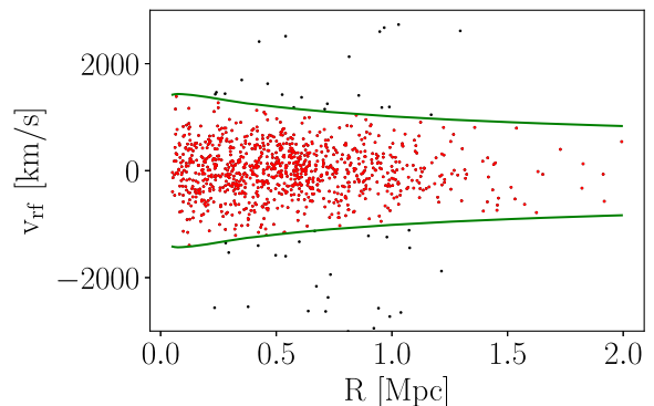
Figure 1. The projected phase space diagram for the composite cluster constructed using those objects having richness in the range 20 \leq \lambda \leq 23.5 . Green lines represent the radially dependent 2.7\sigma_{\text{LOS}} cut used to reject interlopers (indicated by black dots).
