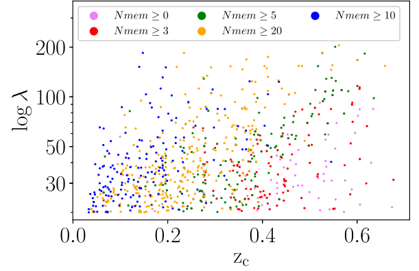
Figure 5. Richness and redshift distribution of clusters having a different number of spectroscopic members.
