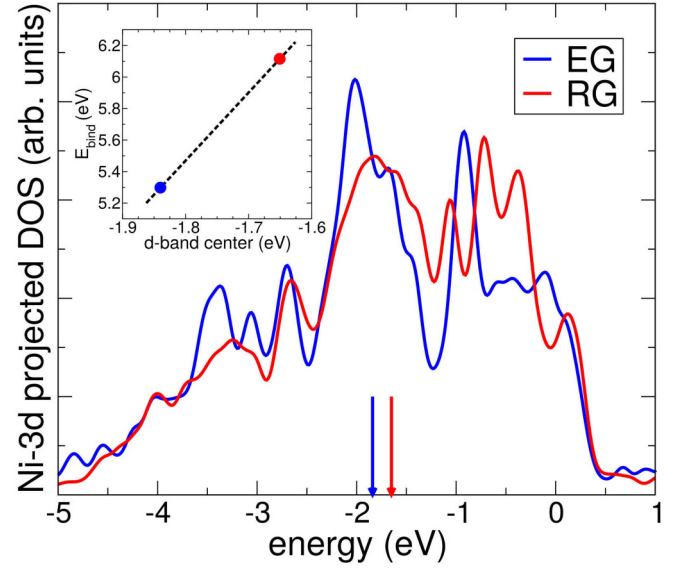
FIG. 6. Density of states (DOS) projected on 3 d orbitals averaged over the Ni atoms nearest to C in the most stable surface sites under EG and RG cover. Arrows indicate the position of d -band center. The correlation between E_{\text{bind}} of C atom and the position of d -band center is plotted in the inset. The Fermi energy is set to zero.
