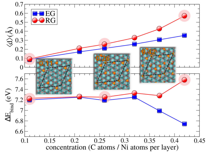
FIG. 8. The mean absolute displacement \langle d \rangle of surface Ni atoms (top) and the incremental binding energy \Delta E_{\text{bind}} for the addition of subsurface C atoms to oh sites (bottom) in EG (blue) and RG (red) at various concentrations \Theta . Top view of RG structures with \Theta = 0.11 , 0.26 , and 0.42 ML are presented in the middle, with the points in graph corresponding to these structures emphasized by semitransparent red circles.
