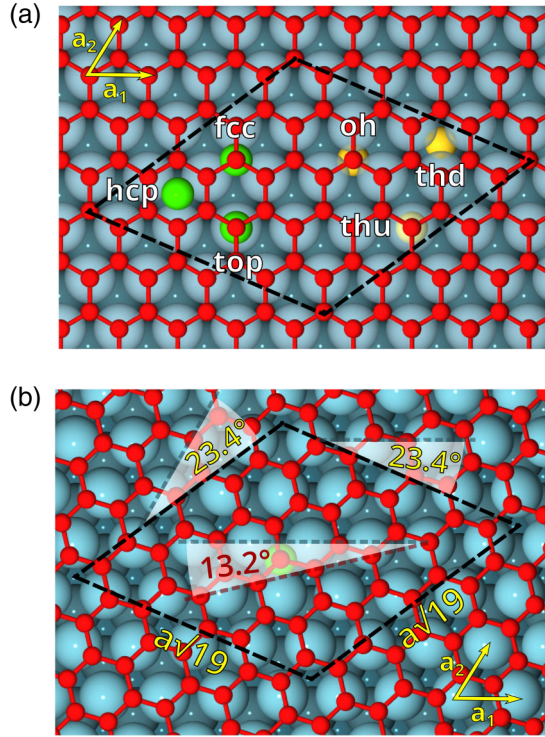
FIG. 5. Structural models of a) EG and b) RG made with (\sqrt{19} \times \sqrt{19}) R 23.4^\circ unit cell. In (a), the surface and the subsurface sites of EG are represented by green and gold spheres, respectively. In (b), the structural details of the unit cell are denoted, in particular: length of the unit cell vectors and the angles between them and \langle 110 \rangle crystallographic directions of nickel. Ni(111) surface lattice vectors are depicted by yellow arrows. The G rotation angle, measured between the \langle 110 \rangle nickel direction and the zigzag direction of G is 13.2^\circ . Green sphere in the middle depicts the most stable surface site for binding C atom directly under RG.
